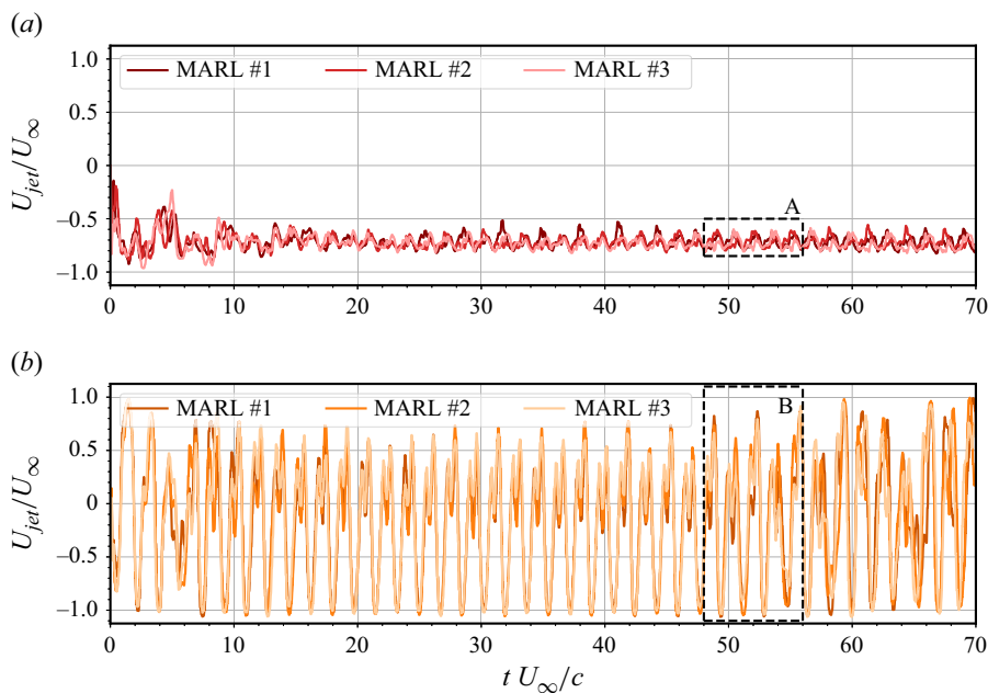
Figure 7. Control actions for (a) DRL NLT-OFF and (b) DRL NLT-ON from the onset of control activation. Only the front jets are shown, with each MARL pseudo-environment represented by a distinct colour.
