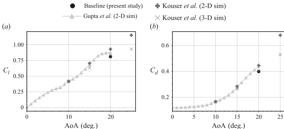
Figure 4. Variation of the mean (a) lift coefficient and (b) drag coefficient with the angle of attack, comparing the present results with the literature.
