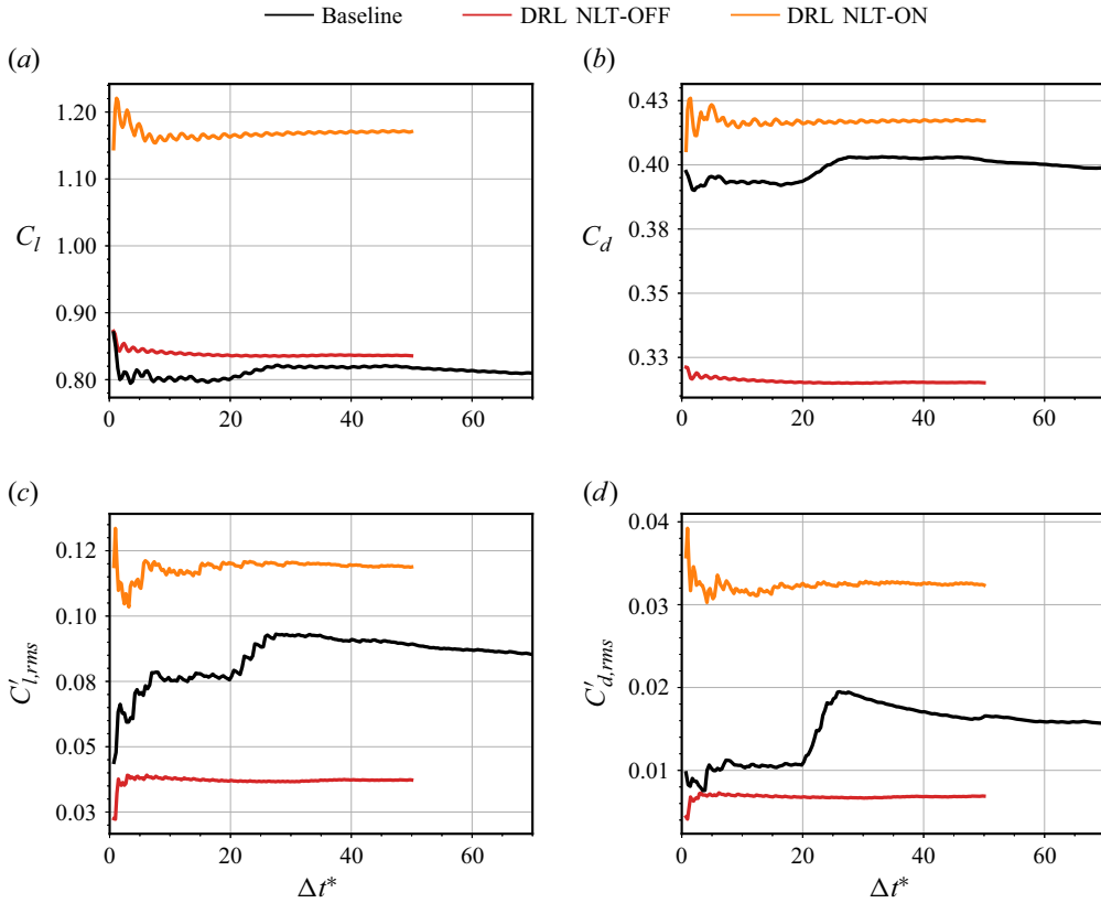
Figure 14. Temporal convergence analysis for the three cases analysed: baseline, DRL NLT-OFF and DRL NLT-ON. Evolution of the (a) lift coefficient, (b) drag coefficient, (c) r.m.s. of the lift coefficient fluctuations and (d) r.m.s. of the drag coefficient fluctuations computed using backward-moving windows of length \Delta t^* from the final simulation time. The window length is \Delta t^* = (t_{end} - t) U_\infty / c , and the accumulated mean is \phi(\Delta t^*) = (1/\Delta t^*) \int_0^{\Delta t^*} \phi(t) dt .
