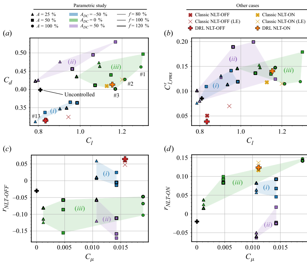
Figure 12. Results of the classic control parametric study compared against the uncontrolled baseline scenario (black '+' markers), the DRL-controlled cases under NLT-OFF (red '+' markers) and NLT-ON (orange '+' markers) and the classic controls derived from the corresponding DRL cases (red and orange 'x' markers): (a) lift coefficient versus drag coefficient; (b) lift coefficient versus r.m.s. of lift coefficient fluctuations; and momentum coefficient versus local reward under (c) NLT-OFF and (d) NLT-ON.
