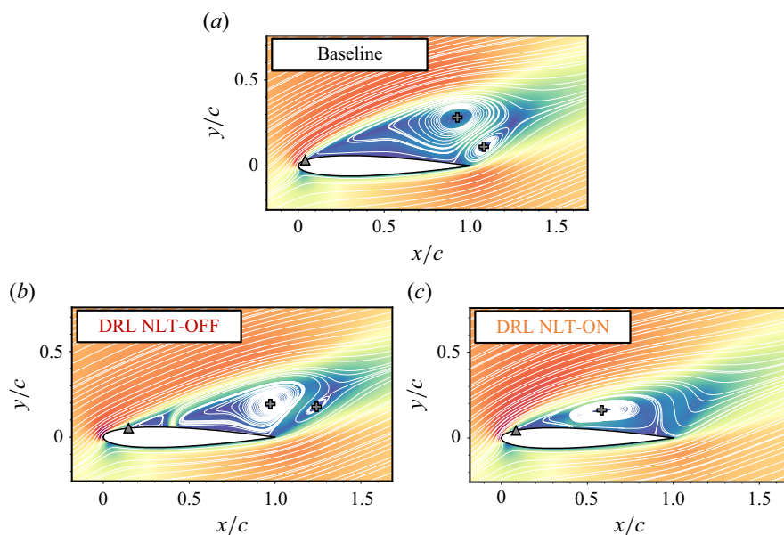
Figure 9. Time-averaged velocity streamlines with the velocity magnitude shown in the background. Results are presented for the (a) baseline, (b) DRL NLT-OFF and (c) DRL NLT-ON scenarios. Crosses indicate the locations of the vortex cores, and triangles denote the flow separation point at the leading edge.
