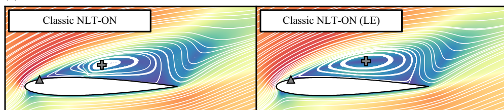
Figure 13. Time-averaged velocity streamlines with the velocity magnitude shown in the background. Classical control cases based on DRL NLT-OFF are shown in (a), while those derived from DRL NLT-ON are shown in (b). Crosses indicate the locations of the vortex cores, and triangles denote the flow separation point at the LE.
