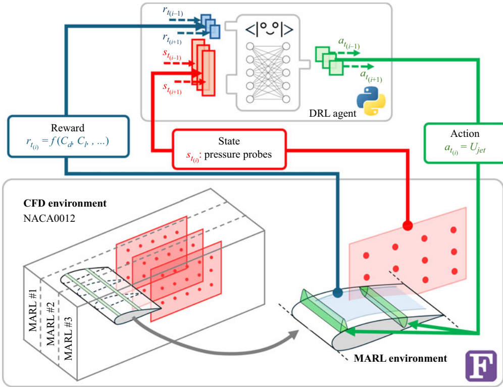
Figure 1. Schematic of the DRL framework showing the MARL strategy.
