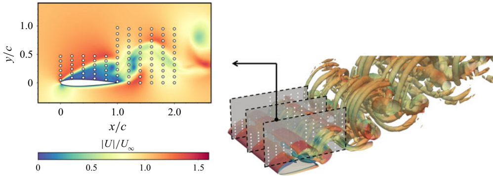
Figure 3. Sensor locations used as the DRL agent state, superimposed on a snapshot of the baseline flow field: zoomed view shows instantaneous velocity magnitude, general 3-D view shows Q-criterion (the second invariant of the velocity gradient tensor) iso-contours Qc^2/U_\infty^2 = 0.1 coloured by velocity magnitude.
