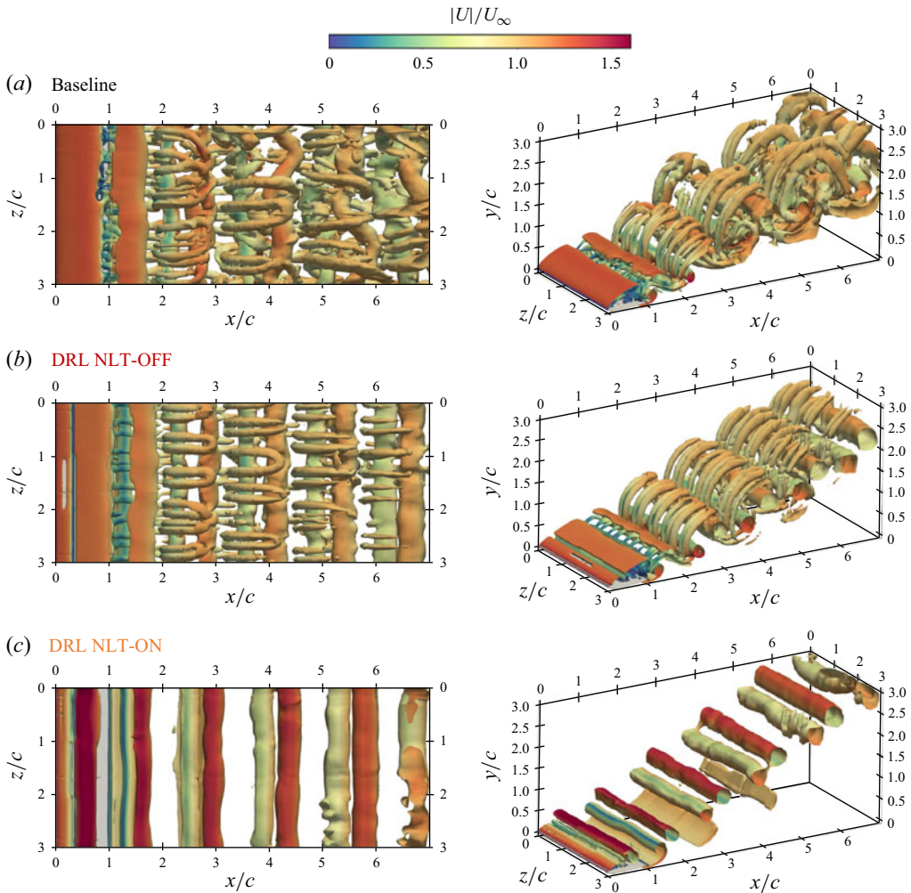
Figure 10. Visualisation of vortical structures using Q-criterion iso-contours Qc^2/U_\infty^2 = 0.1 coloured by velocity magnitude. (a) Baseline, (b) DRL-control under NLT-OFF and (c) DRL-control under NLT-ON. On the left, the top view; and on the right, the perspective view.
