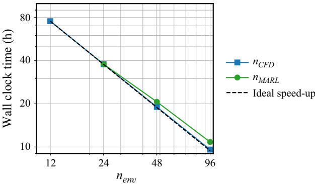
Figure 15. Total wall-clock time (in hours) required for training as a function of the number of CFD simulations and MARL pseudo-environments.
