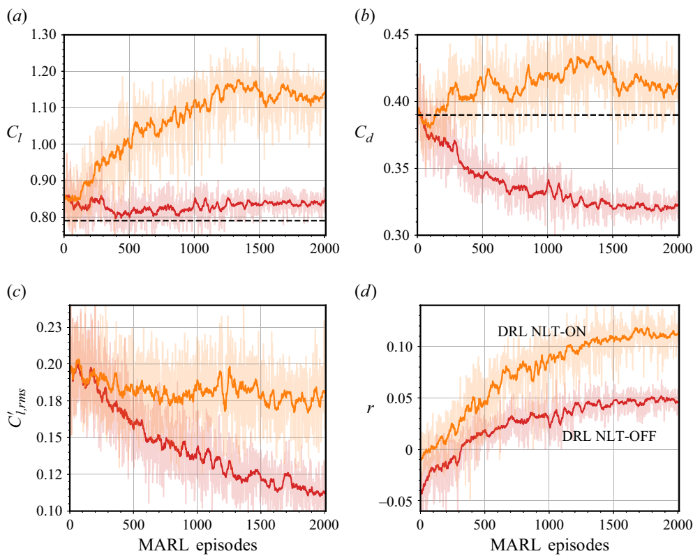
Figure 5. Evolution of the mean (a) lift coefficient, (b) drag coefficient, (c) lift coefficient fluctuations and (d) local reward over the last 5U_\infty/c of each episode during training. In each plot, a moving average is applied to smooth signals, while the individual data points are shown in a lighter, more transparent colour. The dashed black lines in (a) and (b) represent the baseline average value from the non-actuated case.
