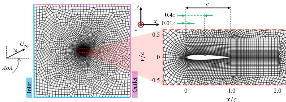
Figure 2. Visualisation of the computational mesh. The full domain is shown on the left, while a zoomed-in view around the wing is displayed on the right. Only the spectral elements are shown, whereas Gauss–Lobatto integration points are not displayed. The red dot indicates the origin of the coordinate system, while the green triangles denote the locations of the jets.
