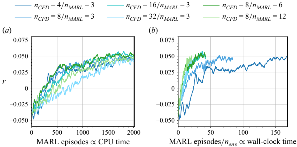
Figure 16. Local reward evolution during training when varying the number of CFD simulations (in blue) and the number of MARL pseudo-environments (in green).
