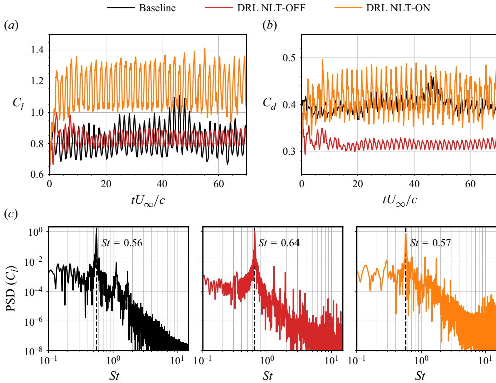
Figure 6. Temporal signals of the (a) lift and (b) drag coefficients when the DRL control is activated during exploitation compared with the baseline signals. (c) Power-spectral densities (PSDs) of the lift coefficient signals.
