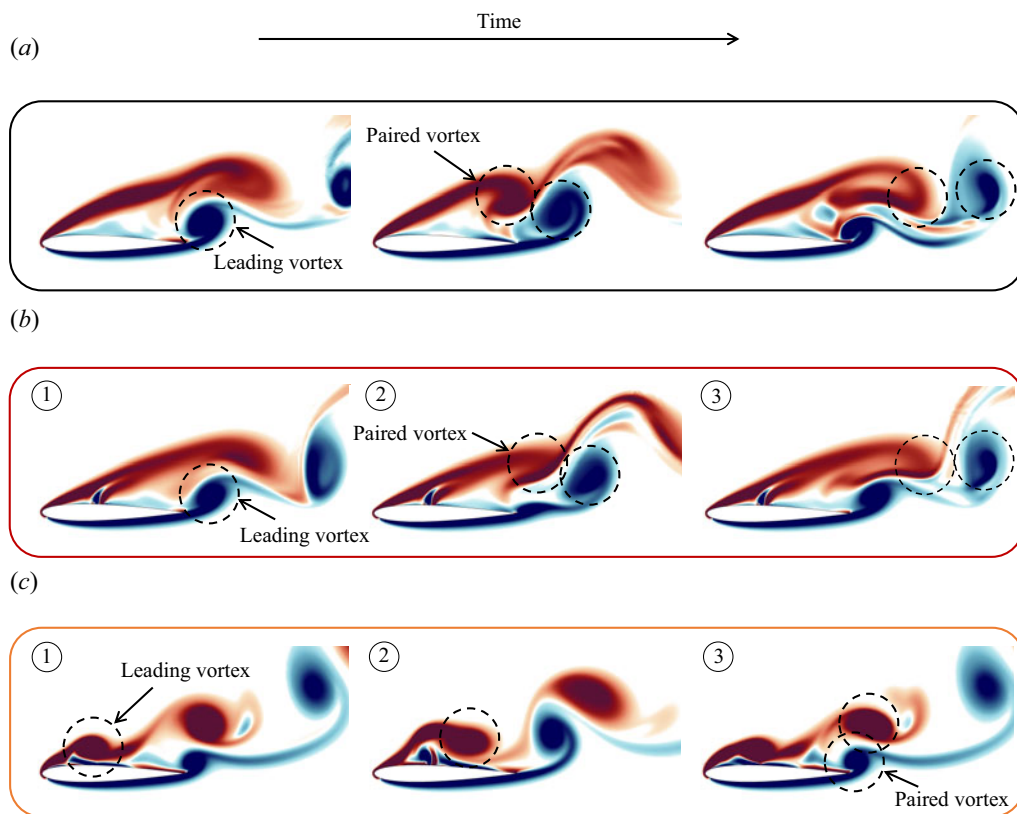
Figure 11. z -Vorticity contours \omega_z c / U_\infty \in [-10, 10] in the x - y plane over a vortex-shedding cycle for the (a) baseline uncontrolled scenario and the DRL-controlled scenarios under (b) NLT-OFF and (c) NLT-ON. Frame numbers 1, 2 and 3 in (b) and (c) correspond to the times highlighted in figures 8(a) and 8(c), respectively.
