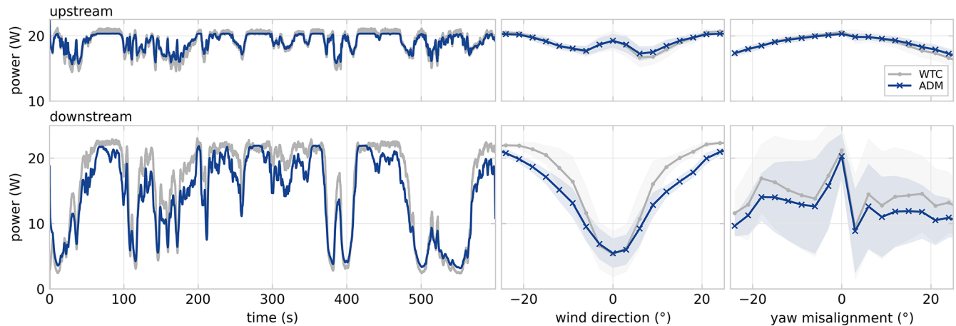
Figure 12. Power predictions with the ADM are compared with experimental data from WTC for the BW30 control setting. The time series fit VAF is 92.1 % for the upstream turbine and 93.3 % for the downstream turbine. The power curves for wind direction and yaw misalignment show the mean and standard deviation in 3^\circ bins. The power variation of the upstream turbine is completely due to variation in yaw misalignment from the open-loop yaw controller. The downstream power is affected both by yaw control on the upstream turbine and by translation for modelling wind direction variation. For larger wind direction magnitudes, the downstream turbine is no longer in waked conditions. The downstream effects of yaw misalignment are clouded by the variation in wind direction, and therefore the power-yaw curves filtered for alignment with the wind direction are presented in Fig. 13.
