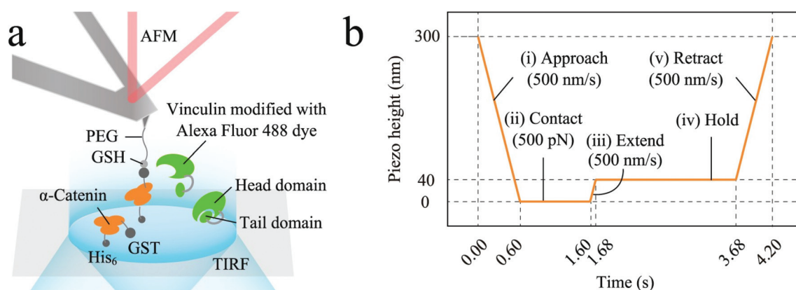
Fig. 5 Example of one of the different AFM/TIRF combined set-ups reported in the literature. (a) \alpha -Catenin molecules (residues 276–634; the mechano-sensitive M1–M3 domain), modified on coverslips, were extended using AFM and simultaneously observed their recruitment of Alexa-labelled full-length vinculin molecules, dissolved in solution, using TIRFM; (b) \alpha -catenin molecules attached to coverslips were tethered by AFM in programmed piezo-height control phases shown in the figure. Reproduced from ref. 174 with permission.
