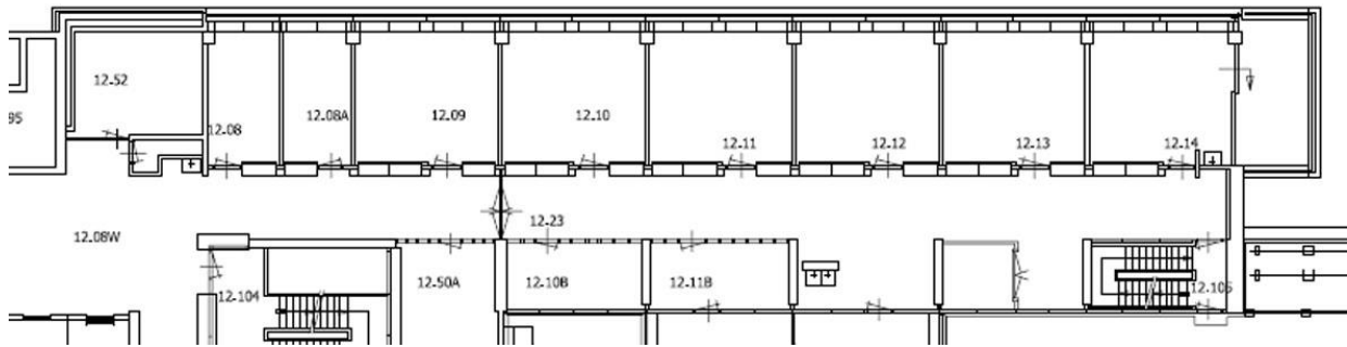
Figure 2: Floorplan of one of the wings of the old building
