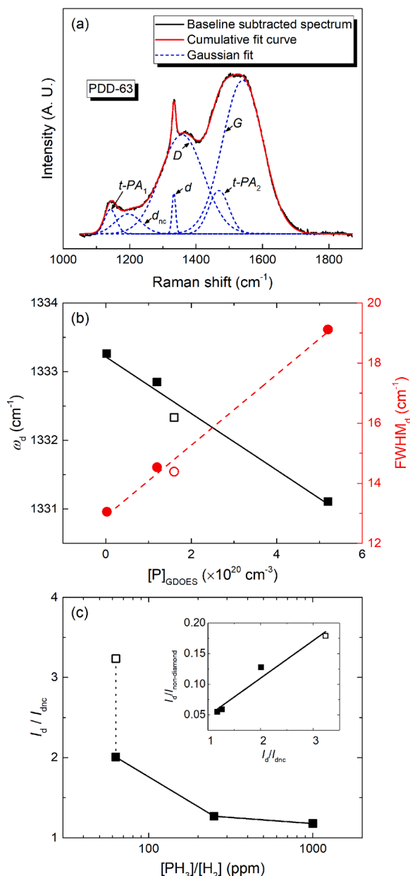
Fig. 2. (a) Baseline subtracted Raman spectrum of the PDD-63 sample (black line), deconvoluted Gaussian peaks (blue dashed lines) contributed from trans -polyacetylene ( t -PA 1 and t -PA 2 ), nanocrystalline diamond ( d nc ), diamond ( d ), and amorphous carbon ( G and D ), and the cumulative curves of the Gaussian peaks (red line). (b) Raman shift ( \omega_d ; black squares, left y-axis) and full width at half maximum (FWHM d ; red circles, right y-axis) of the diamond peak plotted against [P]_{\text{GDOES}} for the layers grown using static (closed symbols) and dynamic gas flow (open symbols). Linear fitting of \omega_d (black solid line) and FWHM d (red dotted line) for [P]_{\text{GDOES}} is also presented. (c) The intensity ratio of diamond to nanocrystalline diamond peaks ( I_d/I_{\text{dnc}} ) for layers grown at different [PH_3]/[H_2] using static (closed squares with solid line) and dynamic (open square with dotted line) gas flows. In the inset, the intensity ratio of diamond to the sum of non-diamond peaks ( I_d/I_{\text{non-diamond}} ) is plotted against ( I_d/I_{\text{dnc}} ) for the layers grown using static (closed squares) and dynamic (open square) gas flows with the linear fitting (solid line).
