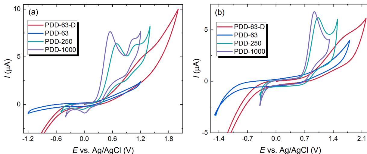
Fig. 6. Cyclic voltammograms of (a) 100 \mu\text{mol L}^{-1} dopamine in 10 \text{mmol L}^{-1} PBS of pH 7.4 and (b) 100 \mu\text{mol L}^{-1} ascorbic acid in 0.1 \text{mol L}^{-1} \text{H}_2\text{SO}_4 recorded on four different PDD samples.
