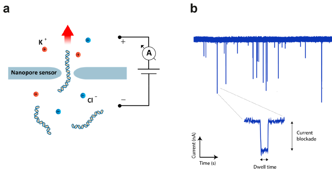
Figure 1. Fundamental principle of nanopore sensing. (a) A nanopore separates two aqueous compartments filled with electrolyte solution (e.g., potassium chloride), and small molecules (e.g., DNA) are electrokinetically pulled through the pore by an applied potential. (b) While passing through the nanopore, the molecule temporarily induces a partial current blockade which is detected by an amplifier. The signature of a single-molecule translocation event is generally characterized by the amplitude of the current blockade, which is proportional to the volume of the molecule in the nanopore, and by the dwell time, which depends on the electrophoretic driving force and transient interactions between the passing molecule and the pore surface.
