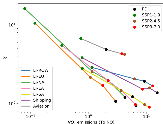
Figure 10. Dependency between \chi and the annual \text{NO}_x emissions (in \text{Tg}(\text{NO}) ). \chi is calculated as the global mean over 5 years. Shown are the results of the seven transport categories (LT-ROW, LT-EU, LT-NA, LT-SA, LT-EA, aviation, and shipping, where LT indicates land transport) for each simulation (colour-coded).
