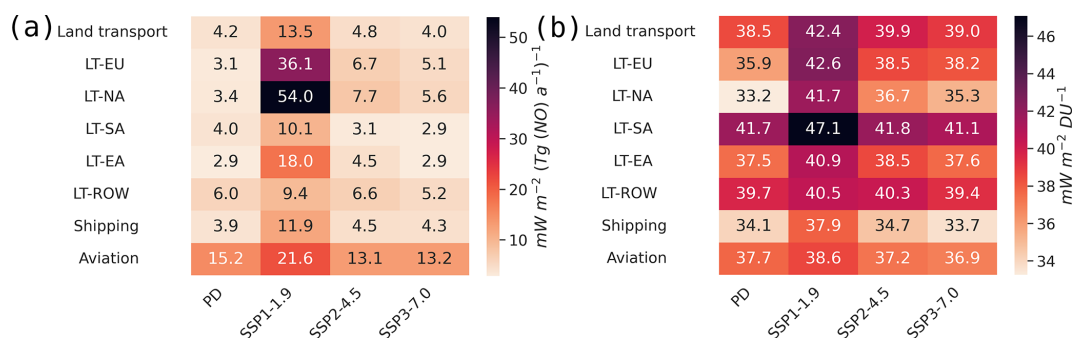
Figure 12. Global averages of R_{Fe} (a, in \text{mW m}^{-2} ((\text{Tg}(\text{NO}) \text{a}^{-1})^{-1}) ) and R_{F_{DU}} (b, in \text{mW m}^{-2} \text{DU}^{-1} ) for the emission sectors land transport, shipping, and aviation as well as for the land transport emissions from specific regions only.
