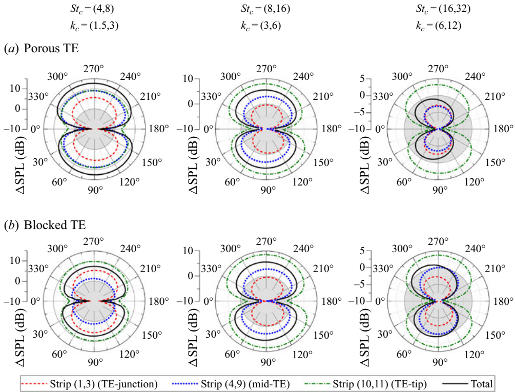
Figure 13. Noise directivity pattern, plotted in terms of the difference between the SPL of permeable (porous and blocked TE) and solid TE cases, i.e. \Delta\text{SPL} = \text{SPL}_{\text{solid}} - \text{SPL}_{\text{permeable}} , for groups of strips at different frequency bands. The grey circle at the centre of the polar plot indicates regions of noise increase.
