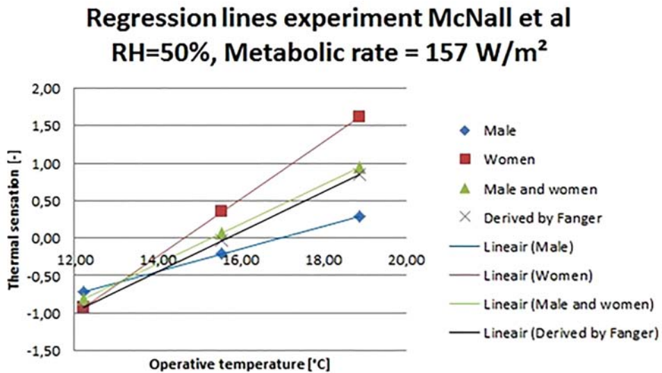
Figure 4. Experimental results McNall et al., metabolic rate of 157 W/m 2 .
