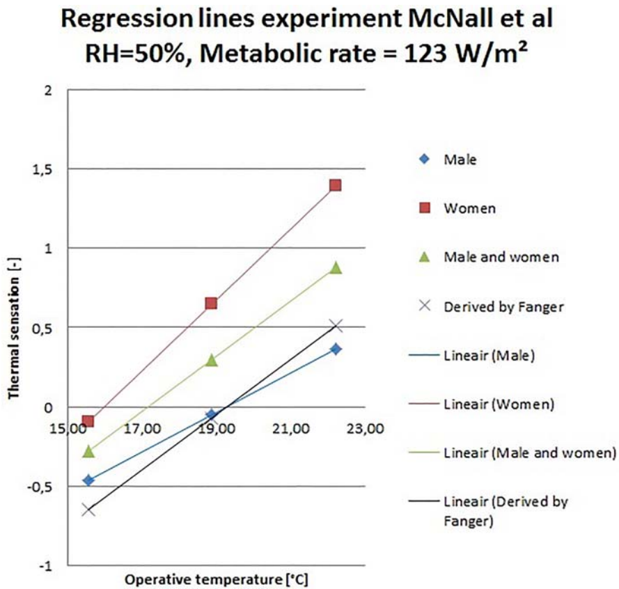
Figure 3. Experimental results McNall et al., metabolic rate of 123 W/m 2 .
