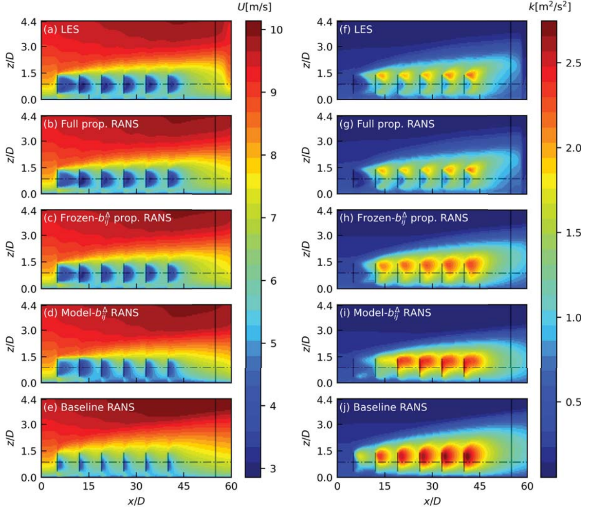
Figure 5: Comparison of x-z planes of U_x (left column) and k (right column) fields at y = 2.5D for 6T7D case simulations. Top to bottom, LES (a, f), full propagation RANS (b, g), frozen- b_{ij}^{\Delta} propagation RANS (c, h), model- b_{ij}^{\Delta} RANS (d, i), and baseline RANS (e, j) fields are shown, respectively. Dark rectangles represent the ADs, and dash-dotted lines indicate the hub heights.
