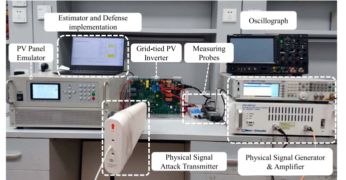
Fig. 3. Experimental setup.
