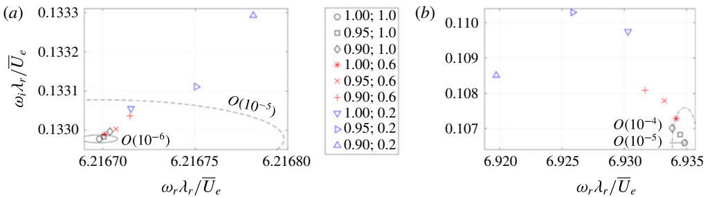
FIGURE 19. (Colour online) Type I (a) and II (b) eigenvalues ( \alpha\lambda_r = 8.2 ) for different domain extrapolation parameters (legend indicates \delta_p ; \delta_o in units of \delta_{mp} ): 10^{-6} (solid line), 10^{-5} (dashed) and 10^{-4} (dash-dotted) neighbourhoods of the eigenvalues with \delta_p = \delta_o = \delta_{mp} .
