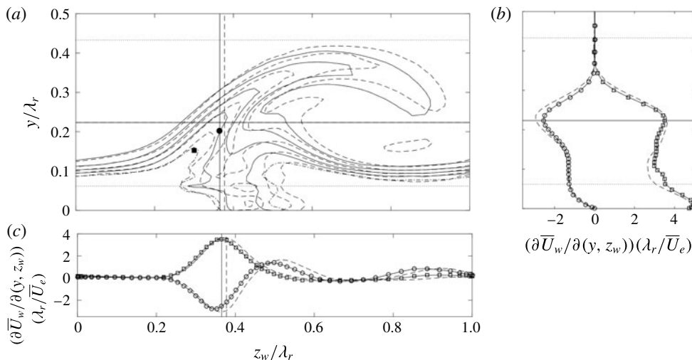
FIGURE 5. (a) In-plane \bar{U}_w -shear magnitude of the weak vortex (solid contours) for N_{fr} = 500 (levels from 0 to 5 with steps of 1 in \bar{U}_e/\lambda_r -units, level 5 \bar{U}_e/\lambda_r is dash-dotted). Position of (\bar{V}, \bar{W}_w) -field saddle point (solid circle), \partial \bar{U}_w / \partial z_w -minimum (solid square) and type I |\tilde{u}_w| -maximum (solid lines). (b) y - and (c) z_w -profiles of \partial \bar{U}_w / \partial z_w (circles) and \partial \bar{U}_w / \partial y (squares) along the straight solid lines in (a). Strong vortex equivalents of the shear profiles and eigenfunction maximum position are given by dashed lines.
