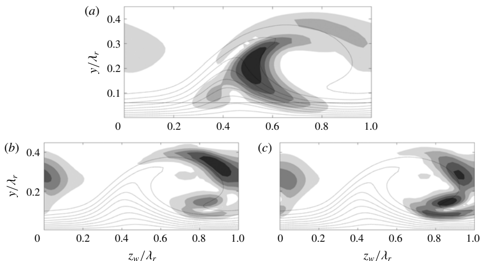
FIGURE 8. |\tilde{u}_w|/\max|\tilde{u}_w| for the type III mode (a, in figure 7a) and the ‘harmonics’ of type II (b,c, respectively IIb, IIc in figure 7b) modes, levels span [1/6, 5/6] with \Delta = 1/6 . Near-wall region (dash-dotted line). \bar{U}_w/\bar{U}_e levels 0.1, 0.2, \dots , 0.9 (dotted).
