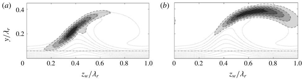
FIGURE 10. |\tilde{u}_w| / \max |\tilde{u}_w| for type I (a) and II (b) (levels span [1/6, 5/6] with \Delta = 1/6 ). 90 \times 90 (filled contours) and 55 \times 55 (dashed) grid resolution. Near-wall region (dash-dotted line). \bar{U}_w / \bar{U}_e levels 0.1, 0.2, ..., 0.9 (dotted).
