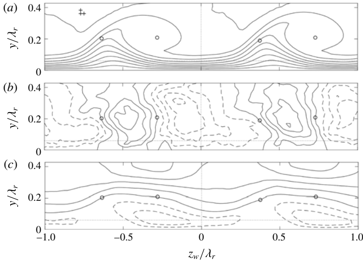
FIGURE 3. (a) \overline{U}_w/\overline{U}_e (10 levels, from 0 to 1), (b) \overline{V}/\overline{U}_e (11 levels, from -0.02 to 0.02 ) and (c) \overline{W}_w/\overline{U}_e (11 levels, from -0.05 to 0.05 ) at constant x_w ( x = 45.6\% chord at z_w/\lambda_r = 0 ), negative contours are dashed. Spatial resolution of experimental data (pluses, \Delta y = \Delta z_w = 0.022\lambda_r ), (\overline{V}, \overline{W}_w) -field centre and saddle point locations (circles, (z_w, y)/\lambda_r = (0.364; 0.202) - (1, 0) , (0.719; 0.209) - (1, 0) , (0.374; 0.190) and (0.731; 0.209) ), domain separation for strong (right) and weak (left) vortex (vertical dotted line z_w/\lambda_r = 0 ), near-wall region (horizontal dotted line y/\lambda_r \leq 0.061 ).
