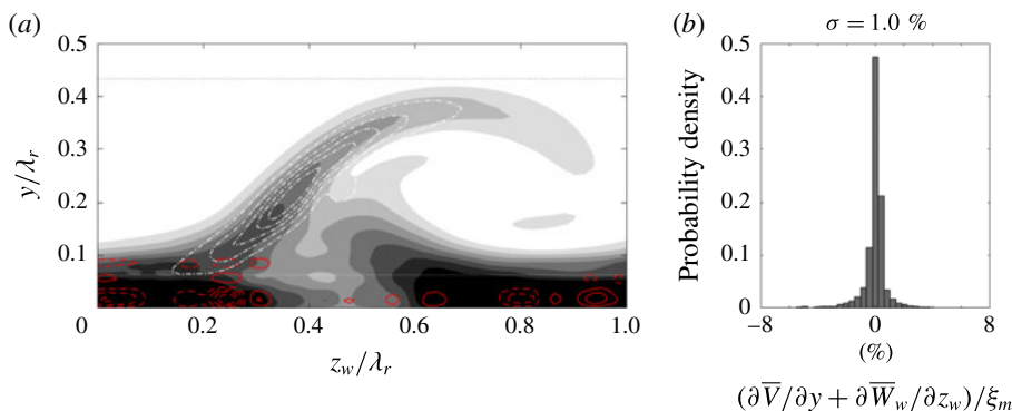
FIGURE 17. (Colour online) (a) In-plane flow divergence (red contours, levels from \pm 2 to \pm 8\% with steps of 2\% of the maximum in-plane \bar{U}_w -shear: \xi_m = 16 \bar{U}_e/\lambda_r , negative levels are dashed). In-plane \bar{U}_w -shear magnitude of the strong vortex for N_{fr} = 500 (8 filled contours from 0 to 7 in \bar{U}_e/\lambda_r -units). |\tilde{u}_w|/\max |\tilde{u}_w| of most unstable type I mode from figure 10 (a) (dash-dotted contours). Near-wall region ( y/\lambda_r \leq 0.061 ) and upper limit PIV domain ( y/\lambda_r = 0.433 ) (dotted lines). (b) Occurrence histogram of divergence values, bar width: 0.4\% .
