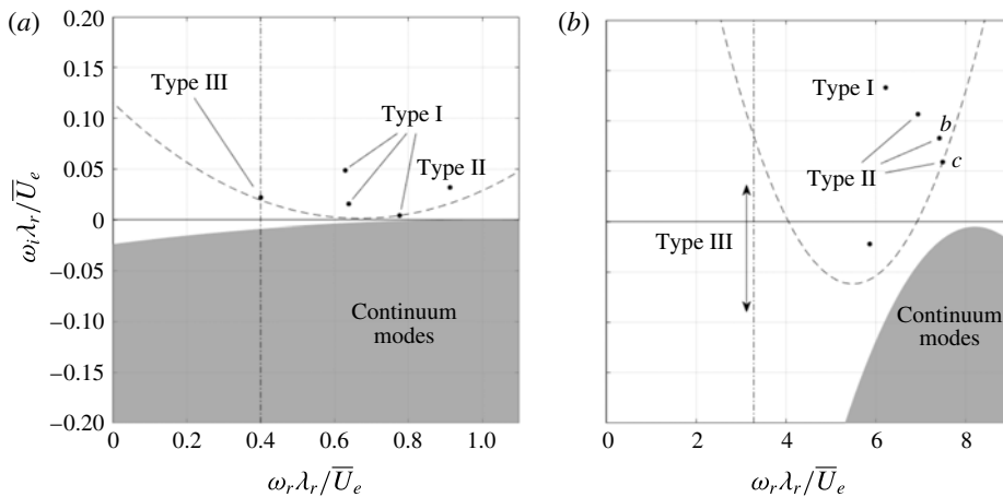
FIGURE 7. Resolved spectra using \omega_g = (0.669 + 2.02i)\alpha/\bar{U}_e , corresponding to \alpha\lambda_r = 1.0 (a) and 8.2 (b). Continuous spectrum (solid surface). Modes dominant in the near-wall region (left of dash-dotted line). \omega_g -centred circle enclosing resolved eigenvalues (dashed line).
