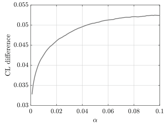
Fig. 7 Illustration of the confidence level (CL) difference (1 - \alpha) - P(\bar{x} \in S_\alpha^{\text{E}}(x) | \mathcal{H}_0) as a function of \alpha
