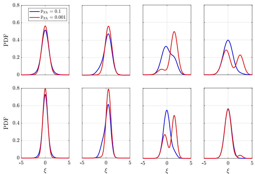
Fig. 1 PDF of \bar{x} under, from left to right, \mathcal{H}_0 , \mathcal{H}_a with b_a = 1 , \mathcal{H}_a with b_a = 3 , and \mathcal{H}_a with b_a = 5 . The top panels correspond to \sigma_{x_0}^2 = 0.5 and \sigma_t^2 = 2 , while the bottom panels to \sigma_{x_0}^2 = 0.25 and \sigma_t^2 = 1 . For the results under \mathcal{H}_a , L_a was set to 0.5
