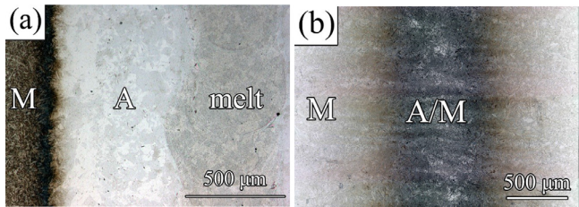
Fig. 1. Microstructures of conditions (a) LINE 9 and (b) LINE 17 in Table 1. M = martensite, A = austenite.
