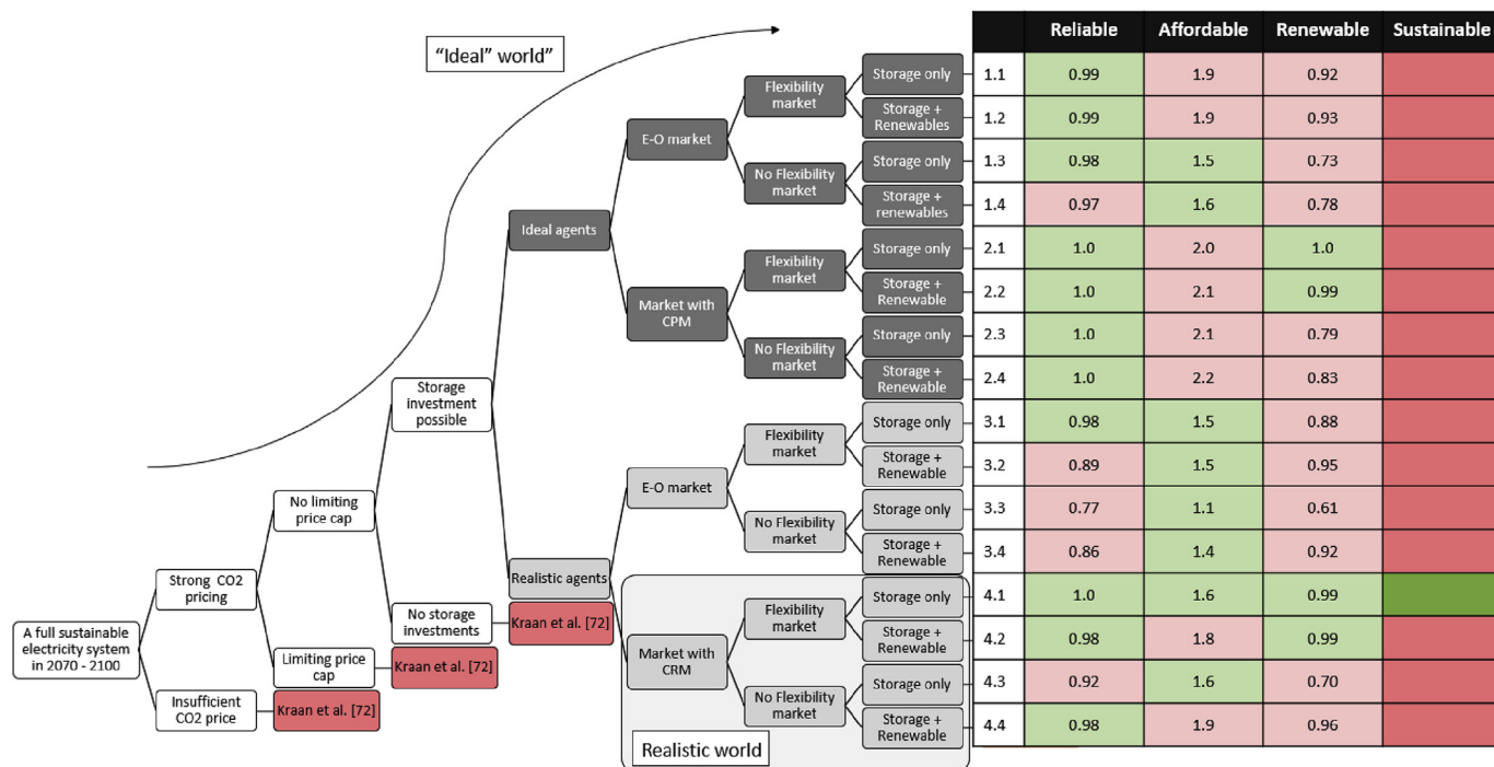
Fig. 6. Results from experiments. The top-branch (dark) of the experiment-tree depicts the experiments with ideal agents, while the lower branch (light-grey) depicts the experiments with more realistic agents. Table shows the average results of the three outcome criteria (reliable, affordable, renewable) over the model runs. Colours depicts whether or not they met the success criterion (red = no, green = yes) based on the defined success criteria. Far right hand column shows result for the overall success criterion: a fully sustainable electricity system in the period 2070 to 2100. Experiment 1.1, 3.1 and 4.1 are treated more extensively in Section 5.1 and subsequently in Figs. 7–9. Graphs show the three outcome parameters, reliability, affordability and renewable ratio; the thick line depicts the median while the shaded areas depict the 25% and 75% percentiles for the models runs. (For interpretation of the references to colour in this figure legend, the reader is referred to the Web version of this article.)
