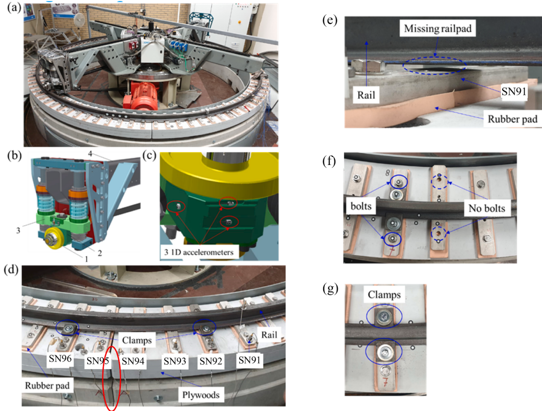
Fig. 1. V-Track and experimental setup for ABA measurement. (a) V-Track test rig; (b) structure of wheel assembly: 1) wheel, 2) axle box, 3) guiding block, 4) steel frame; (c) accelerometers for ABA measurement; (d) track structure overview for a section of V-track (the red oval indicates the gap between SN94 and SN95); (e) missing railpad at SN91; (f) missing sleeper bolts at SN94; (g) top view of fastening clamps. (For interpretation of the references to colour in this figure legend, the reader is referred to the web version of this article.)
