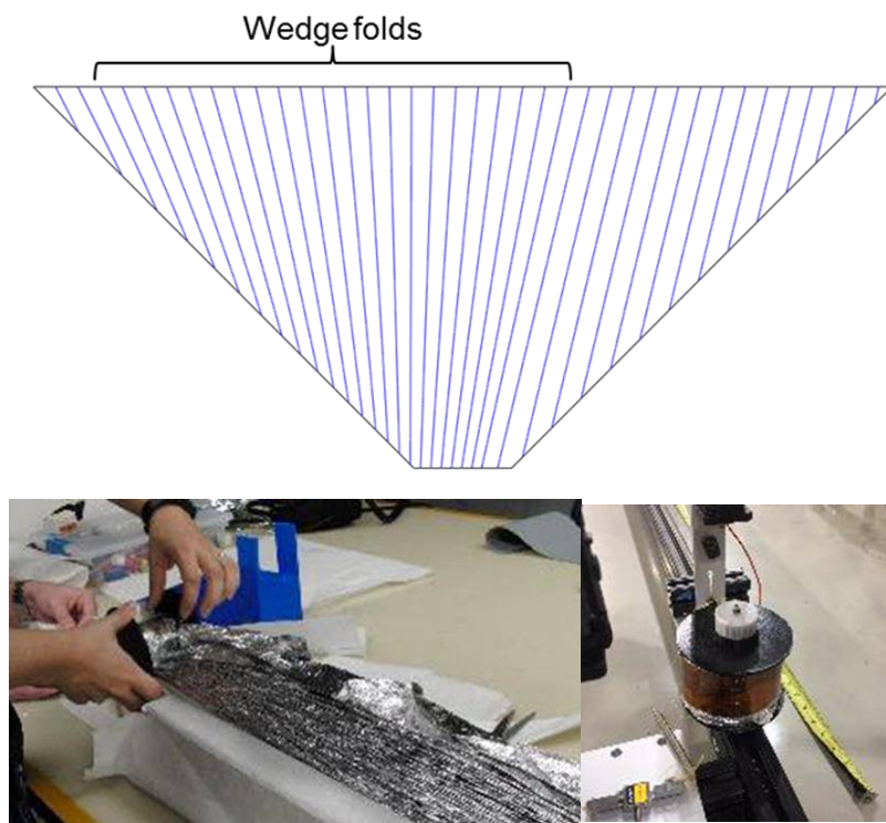
Figure 10. ACS3 sail quadrant folding scheme and spooling process.
