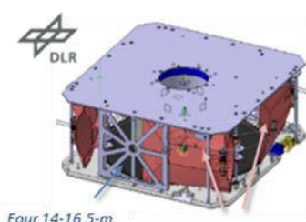
'Guide shell' feature stabilizes transition of boom cross section during deployment.
