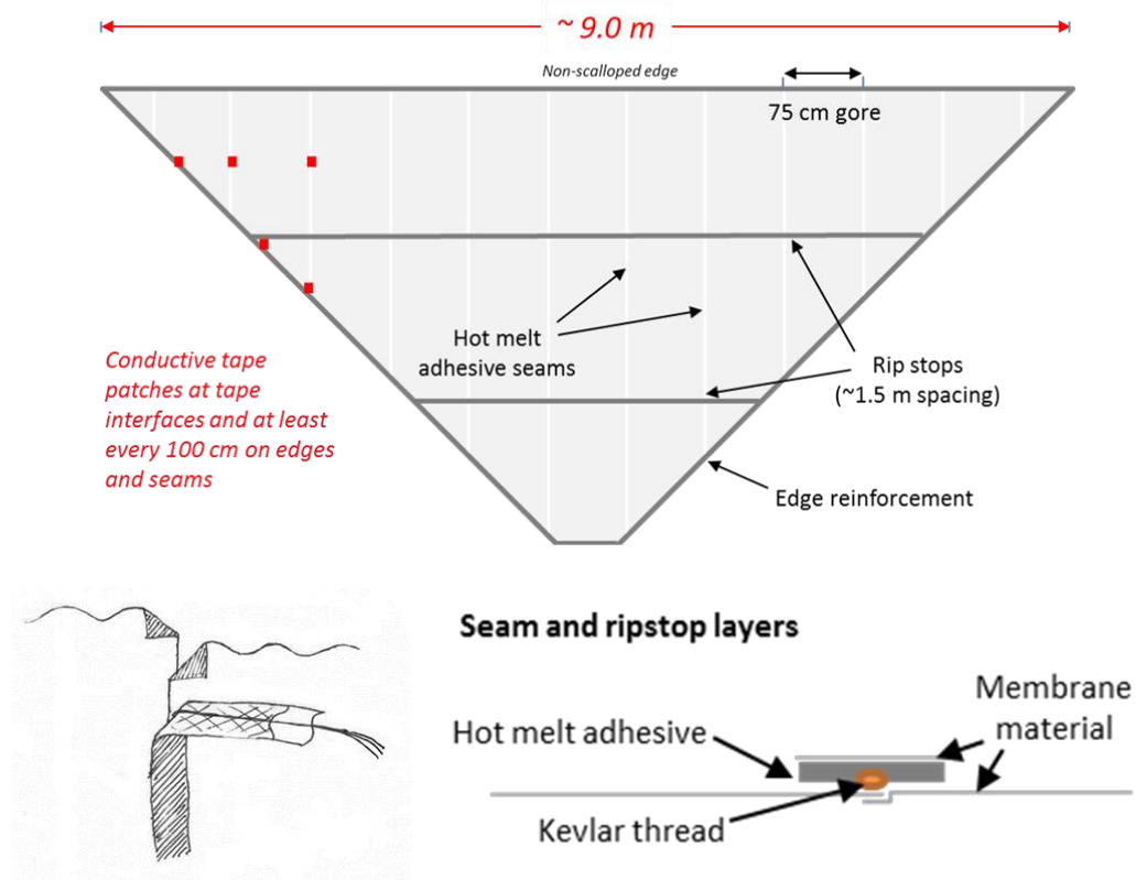
Figure 9. ACS3 solar sail quadrant design and seam construction.
