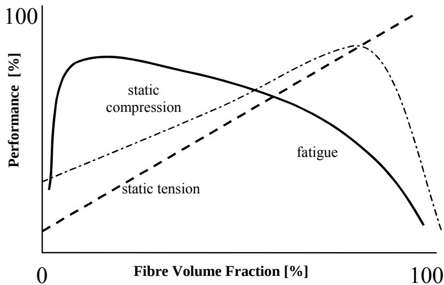
Figure 7: Influence of fibre volume fraction on performance
