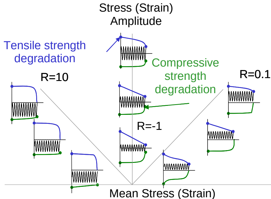
Figure 63: Schematic summary of strength degradation trends from various OPTIMAT laminates and geometries, in CLD format
