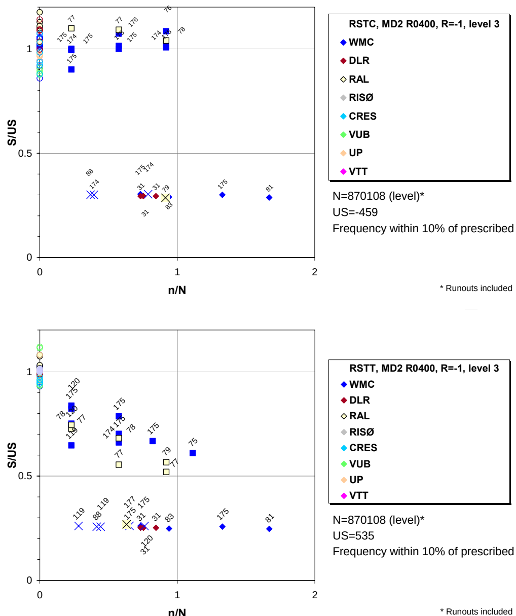
Figure 62: Example residual strength plots, reproduced from 225
