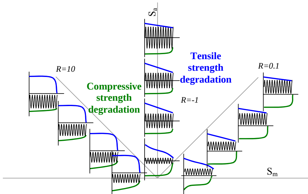
Figure 87: Summary of residual strength trends
