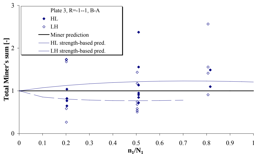
Figure 76: Two-block test results for R=-1
