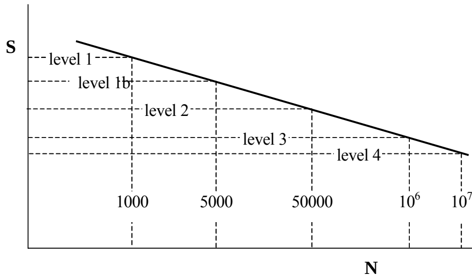
Figure 59: Standard OPTIMAT load levels
