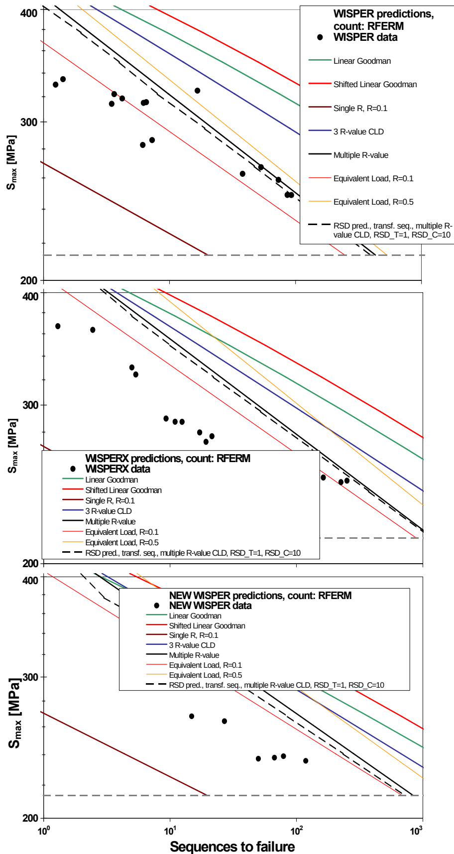
Figure 88: Life predictions using Rainflow-equivalent Range-mean counted spectra and various CLDs
