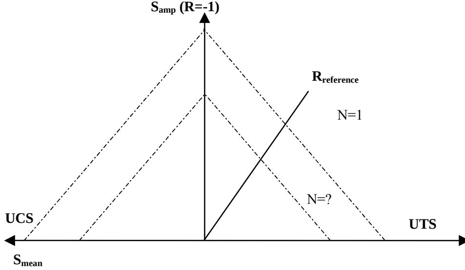
Figure 14: Equivalent load method CLD
