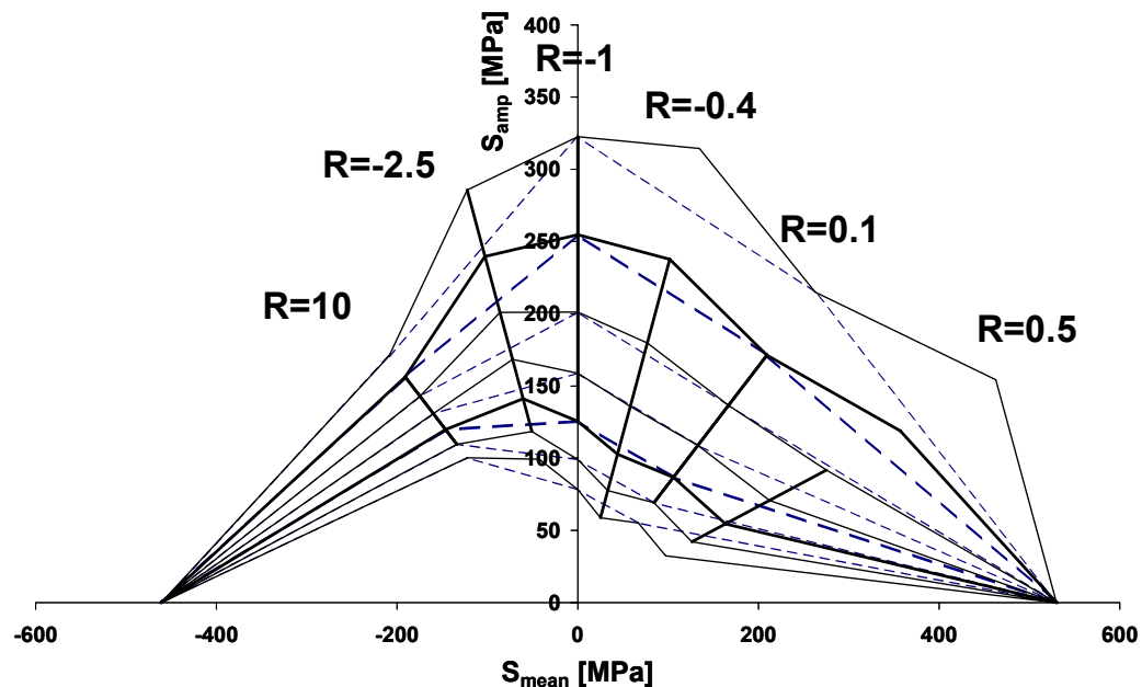
Figure 92: Comparison of 3 R-value (blue dotted) and 6 R-value CLDs
