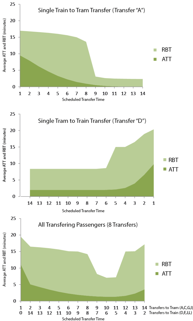
3 FIGURE 6 Average additional travel time and reliability buffer time for passengers of 4 "Transfer A" (top), passengers of "Transfer D" (middle) and all transferring 5 passengers (from all 8 transfers, bottom).
