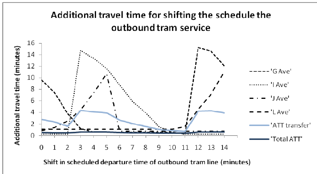
15 16 FIGURE 7 Additional travel time for shifting the schedule of tram line 9 (westbound) in 17 Den Haag. The transfer point is Den Haag HS.
