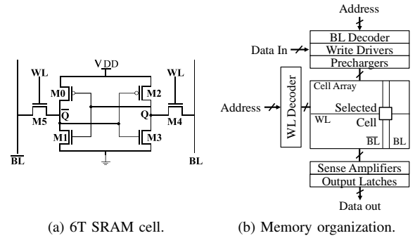
Fig. 1. Memory model.
