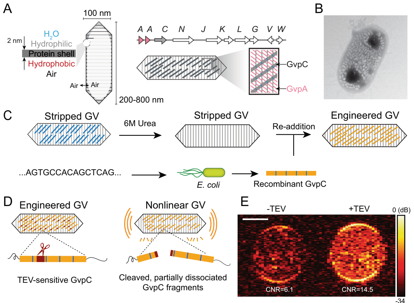
Fig. 3. GV engineering . (A) GV hollow protein nanostructure, gene cluster encoding GVs and surface arrangement of the GV shell proteins GvpA and GvpC. Adapted with permission from (Maresca et al., 2018b). (B) Heterologous expression of gas vesicles in E. coli . Adapted with permission from (Bourdeau et al., 2018). (C) GvpC bioengineering pipeline, adapted with permission from (Maresca et al., 2018b). (D) Design of an acoustic biosensor of Tobacco Etch Virus (TEV) protease activity. Adapted with permission from (Lakshmanan et al., 2020). (E) Nonlinear ultrasound imaging of acoustic biosensors of TEV activity. Scale bar = 1 mm. Adapted with permission from (Lakshmanan et al., 2020).
