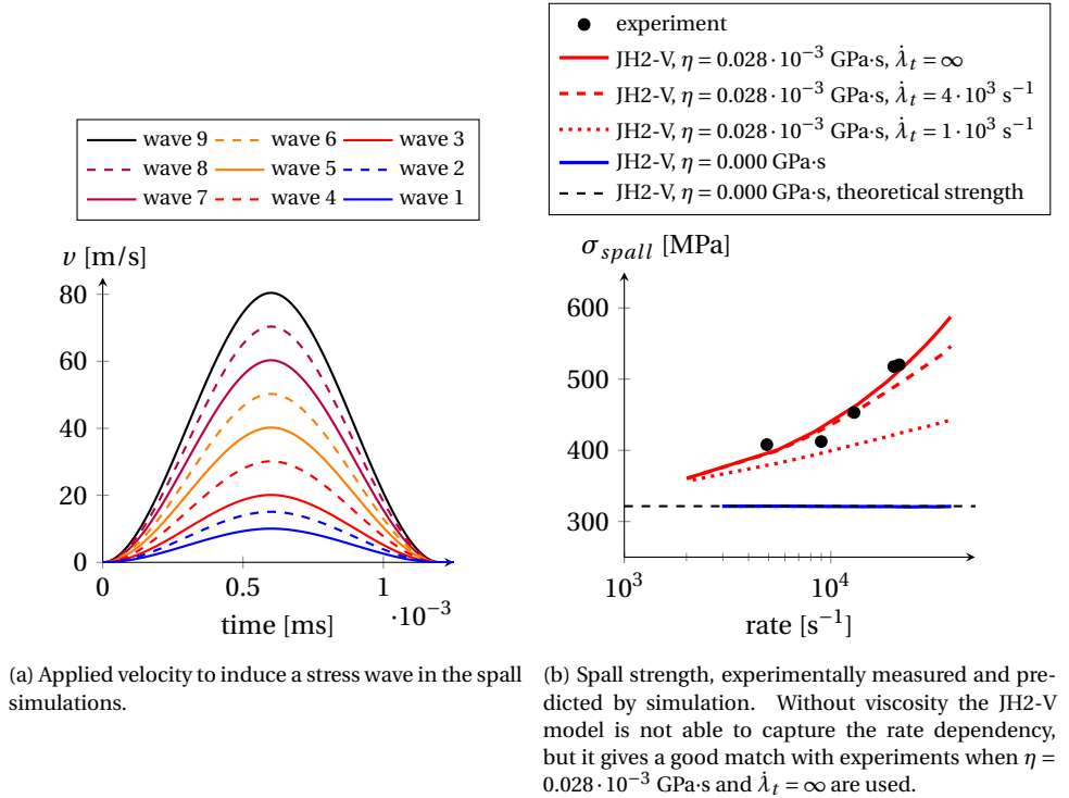
Figure 3.2: Spall test on alumina ceramic, comparing experiments to simulations.
