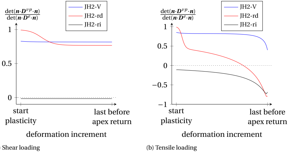
Figure 2.3: Single element tested under pure shear and uniaxial tension. The graphs show the normalized determinant of the acoustic tensor. A negative value indicates a loss of ellipticity of the boundary value problem. This will lead to mesh-dependent results.
