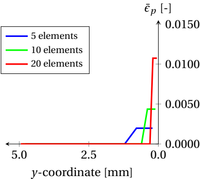
(c) Equivalent plastic strain profile along the tapered bar axis. An increase in equivalent plastic strain can be found for decreasing mesh size.
