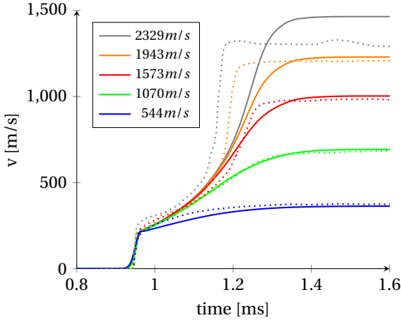
Figure 3.8: Simulation results for a plate impact test on alumina ceramic. The parameter set used to obtain Figure 3.5 was also used here, but with d_1 = 0.050 and \dot{\lambda}_t = 40000 \text{ s}^{-1} . The dotted lines show the experimental results from [55], the solid lines are simulation results.
