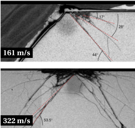
(c) Silicon carbide ceramic after sphere impact, pictures are obtained from [58]. A quasi-plastic zone is found below the projectile, but the material is not comminuted.
