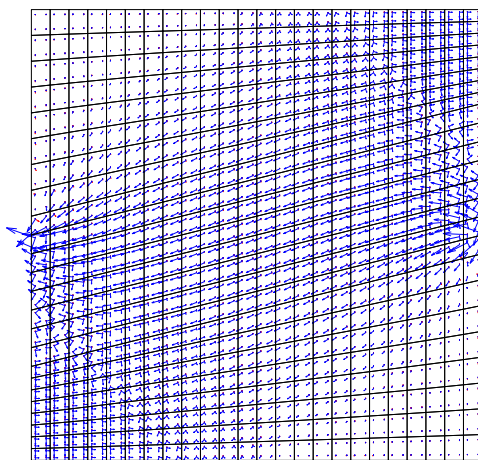
(c) Principal stress direction, elastic loading, upward slanted mesh.
