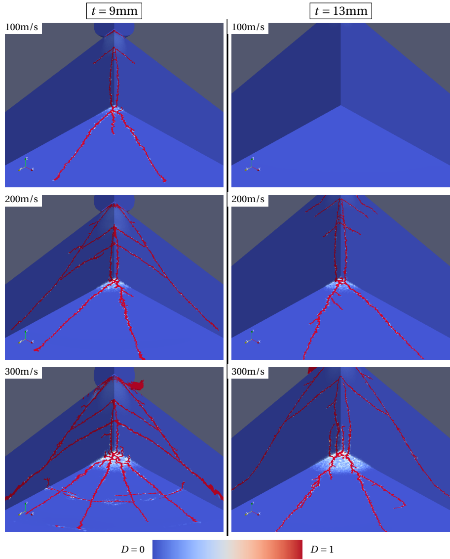
Figure 4.13: Sphere impact simulations performed in 3d with the same set-up as the experiments from DRDC. The simulations are terminated after 10\mu\text{s} of simulated time.
