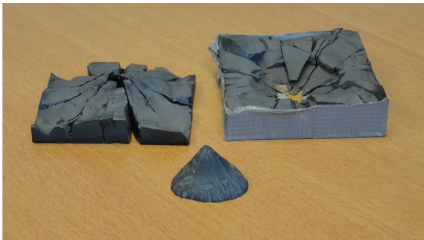
Figure 1.3: Silicon carbide ceramic tile, subjected to a single projectile impact. Cone cracking and radial cracking in the ceramic target is clearly visible. (E. Carton, TNO Laboratory for Ballistic Research, personal communication)
