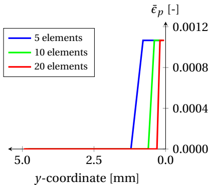
(c) Equivalent plastic strain profile along the tapered bar axis. The equivalent plastic strain can be found to be equal for all mesh sizes.
