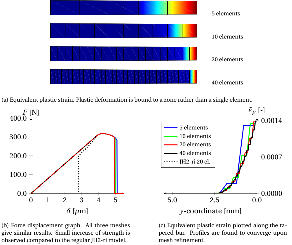
Figure 2.10: Tapered tensile bar results for the JH2-V model.
