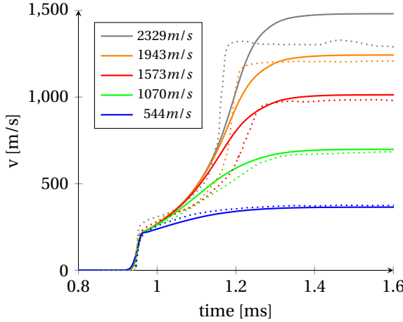
Figure 3.19: Simulation results for a plate impact test on alumina ceramic. The parameter set for the spall test is used, but with the newly proposed failure strain formulation and \dot{\lambda}_t = 40000\text{s}^{-1} . The results are very similar to those obtained with the original JH2 formulation with d_1 = 0.500 and \dot{\lambda}_t = 40000\text{s}^{-1} , from Figure 3.9. The dotted lines show the experimental results from [55], the solid lines are simulation results.
