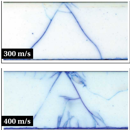
(b) Alumina ceramic after sphere impact, pictures are obtained from [57]. Comminution of ceramic directly below the projectile is absent.
