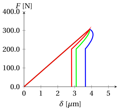
(b) Force displacement graph. Localization upon mesh refinement is clearly visible.
