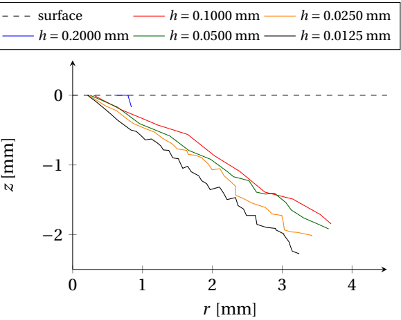
(a) Mesh dependency study, variable element size h at the contact surface. The target interior element size is the same for all cases. For a coarser mesh the radius of the surface ring crack is larger, as is the cone crack angle.
