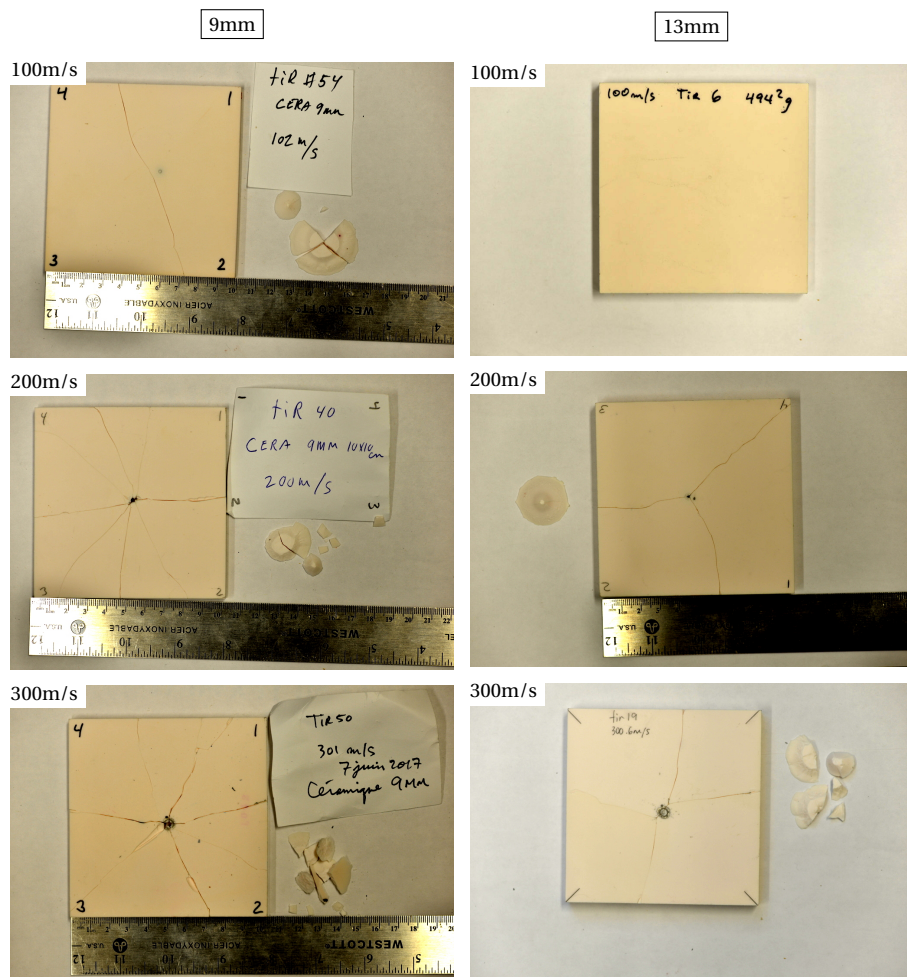
Figure 4.3: Experimental results of sphere impact on alumina ceramic. Two tile thicknesses are considered for three impact velocities. For all test cases the target front surface is shown, with (parts of) the cone next to it. The 13mm 100m/s cases did not result in cone formation.
