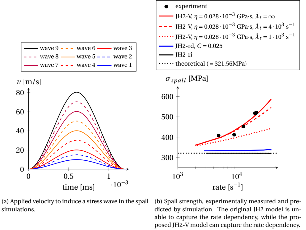
Figure 2.29: Spall test on alumina ceramic, comparing experiments to simulations.
