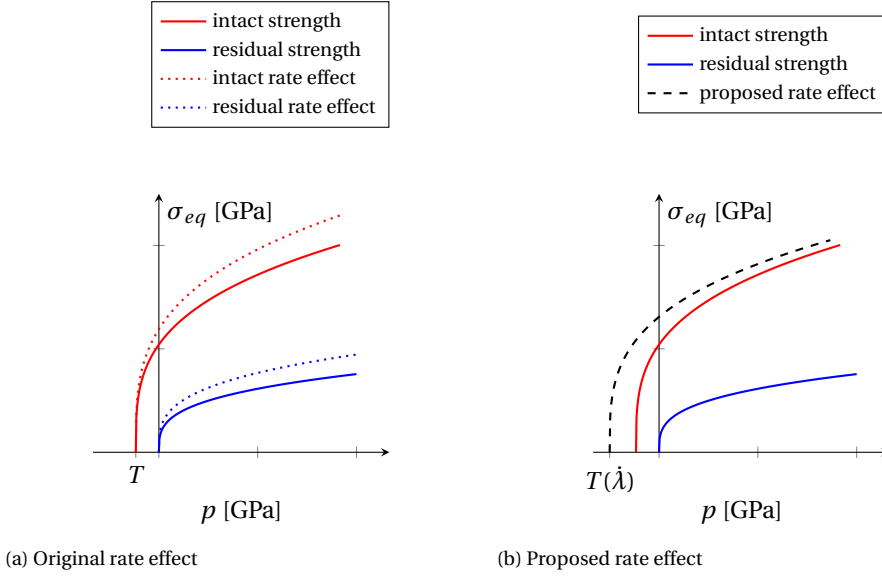
Figure 2.1: Deviatoric strength \sigma_{eq} of the Johnson-Holmquist-2 material model plotted as function of pressure p . Figures show the original and proposed rate effects. Note the relatively large increase in strength under tension and the minimal increase under compression for the proposed model.
