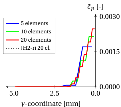
(c) Equivalent plastic strain plotted along the tapered bar axis. The profiles are found to converge upon mesh refinement.
