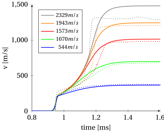
Figure 3.9: Simulation results for a plate impact test on alumina ceramic. The parameter set used to obtain Figure 3.5 was also used here, but with d_1 = 0.500 and \dot{\lambda}_t = 40000\text{s}^{-1} . The dotted lines show the experimental results from [55], the solid lines are simulation results.
