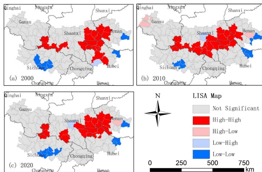
Figure 5. The spatial agglomeration of ecosystem health based on Rook contiguity from 2000 to 2020.
