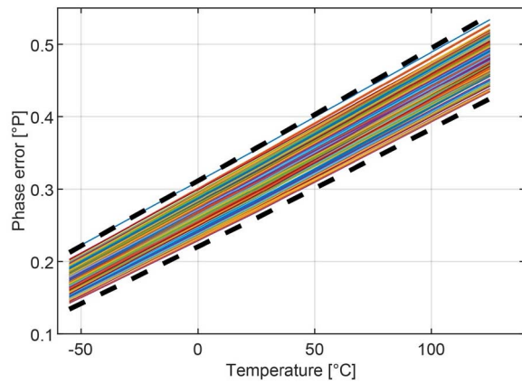
Fig. 9. Simulated additional phase shift due to the CCO non-linearity at -55^\circ\text{C} , 25^\circ\text{C} , and 125^\circ\text{C} (Monte-Carlo process + mismatch). Dashed line: 3\sigma values.
