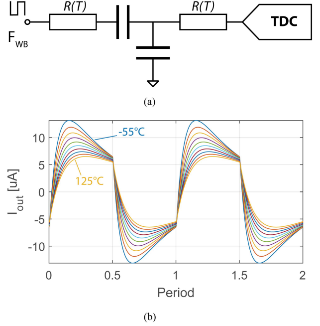
Fig. 2. (a) Single-ended WB. (b) Output waveform of a single-ended WB at different temperatures.
