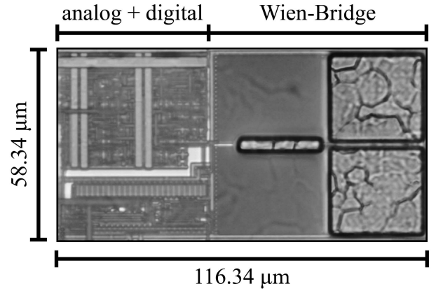
Fig. 15. Chip photograph.
