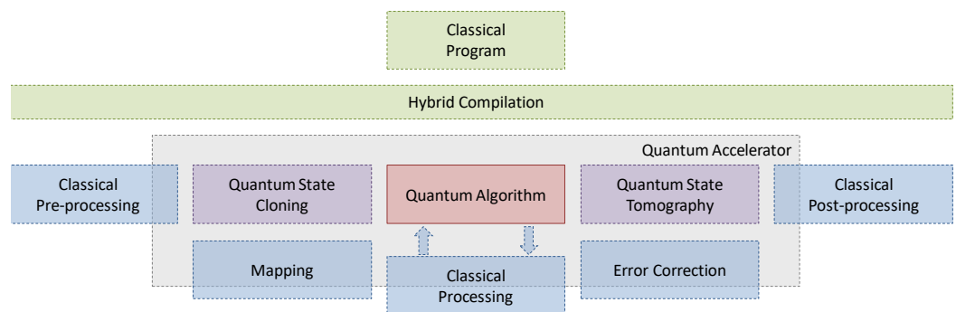
Figure 8. Quantum Algorithm (block with solid outline) and interfacing software architecture.
