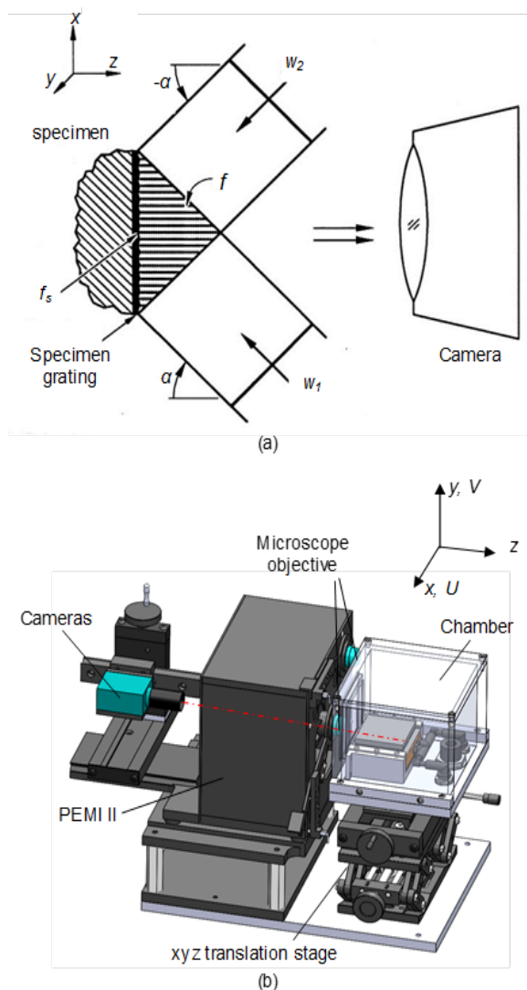
Figure 3.15: Schematic illustration of (a) the principle of moiré interferometry and (b) the optical/mechanical configuration of an advanced portable moiré system.
