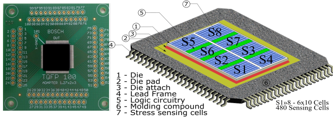
Figure 6.2: TQFP Mounted on a PCB Test Vehicle.
