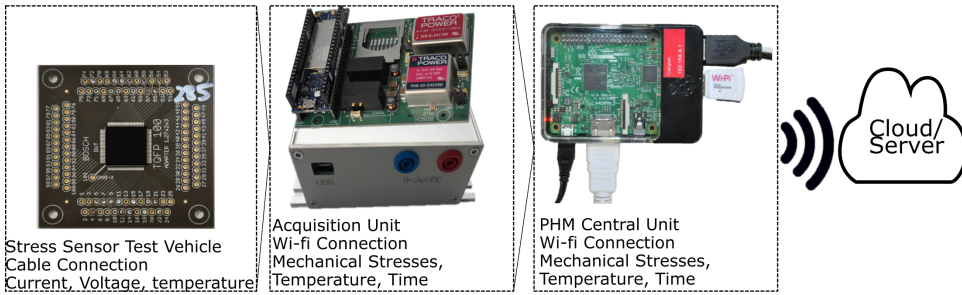
Figure 5.2: Data Flow representation. On each chart is described the electronic unit, the connection, and the data output. Each Test Vehicle is connected to an AU by wires that are able to read out the data from all eight sensors. Up to 5-6 AUs are connected through Wi-Fi to the Raspberry Pi. The cloud or the server collects the data from the Raspberry Pi through a data pipeline.
