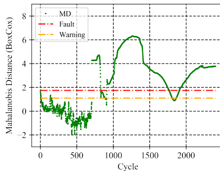
Figure 5.12: Classic threshold MD applied to TQFP stress sensor data. The fault is detected around 850 Cycles.
