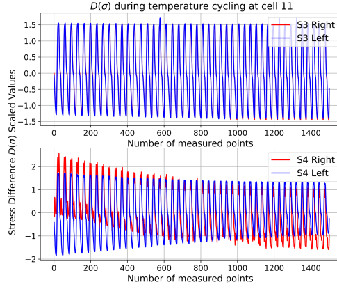
Figure 4.17: Stress difference evolution of the delamination during temperature cycling of the Sample 2.
