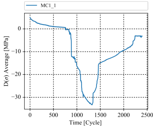
Figure 6.6: Normal in-plane relative stress difference average along all 480 Cells for MC1_1 Sample.
