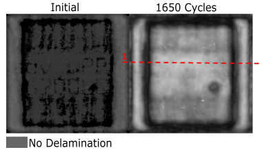
Figure 5.10: SAM of MC1_2 in discrete time. No delamination is present and one cross-section is performed at the end of the experiment, after 1650 Cycles.
