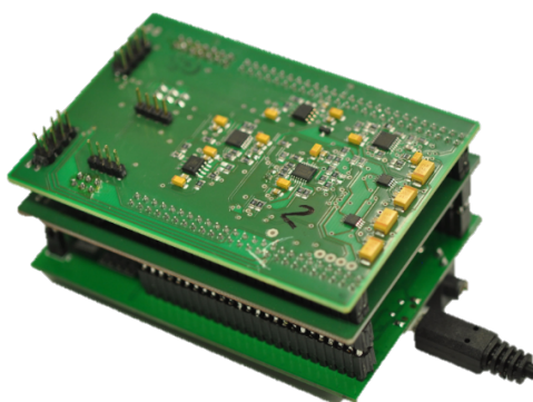
Figure 3.4: Data acquisition unit. The board consists of a microcontroller, power source and logic board.
