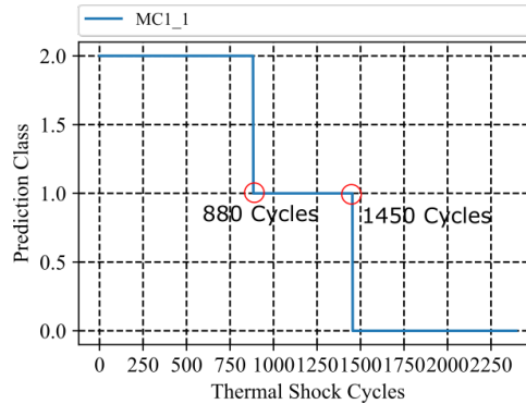
Figure 5.13: Prediction Class with K-Means Clustering method. 2 - represents the health state; 1 - the delamination between molding compound and copper pad; 0 - delamination between the adhesive and silicon die.
