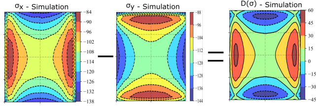
Figure 6.10: TQFP component level mechanical stress at the top of the die. Loading condition used in the simulation is an environmental temperature of -40^\circ and 150^\circ . The stress values at -40^\circ are extracted from 150^\circ stress values.
