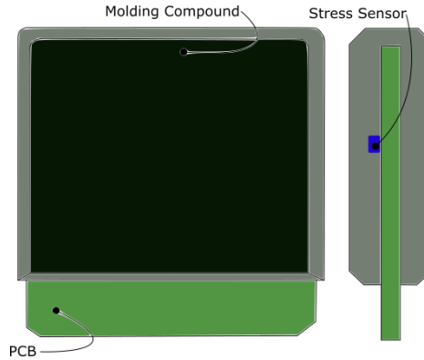
Figure 4.8: Geometry representation of the Outer molded electronic control unit.
