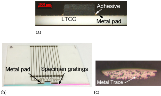
Figure 3.14: (a) Specimen cross section, (b) the replicated specimen gratings and (c) the embedded metal trace.
