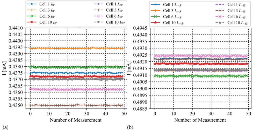
Figure 3.7: Representative averaged current values obtained at room temperature: (a) the average of I_{0^\circ} and I_{+90^\circ} of the pMOS current mirror and (b) the average of I_{-45^\circ} and I_{+45^\circ} of the nMOS current mirror.
