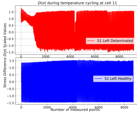
Figure 4.15: Stress evolution of the delamination during temperature cycling of the Sample 1 S1 cell 11 in comparison of the same sensor in a healthy ECU with the same conditions.
