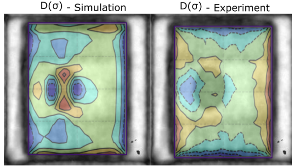
Figure 6.14: MC1_1 TV overlay picture of stress difference on top of SAM image. Both simulation and experiment gives a very good indication where there is still contact underneath the die.
