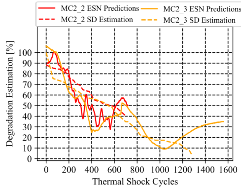
Figure 5.18: Degradation estimation ESN Output vs SD Estimation.
