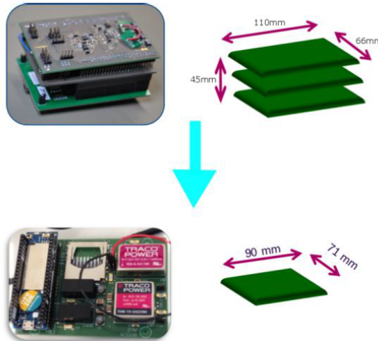
Figure 6.3: Acquisition unit downsizing. The three boards from the previous AU are compressed in a single board.
