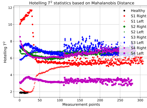
Figure 4.30: Hotelling T2 statistics in the reduced space at room temperature during delamination. The red line corresponding to the same sensor but mirrored can identify a similar behavior, but opposite sign.
