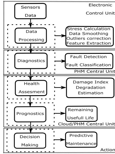
Figure 5.1: Algorithm flowchart that depicts the workflow of the PHM methodology and the corresponding hardware.
