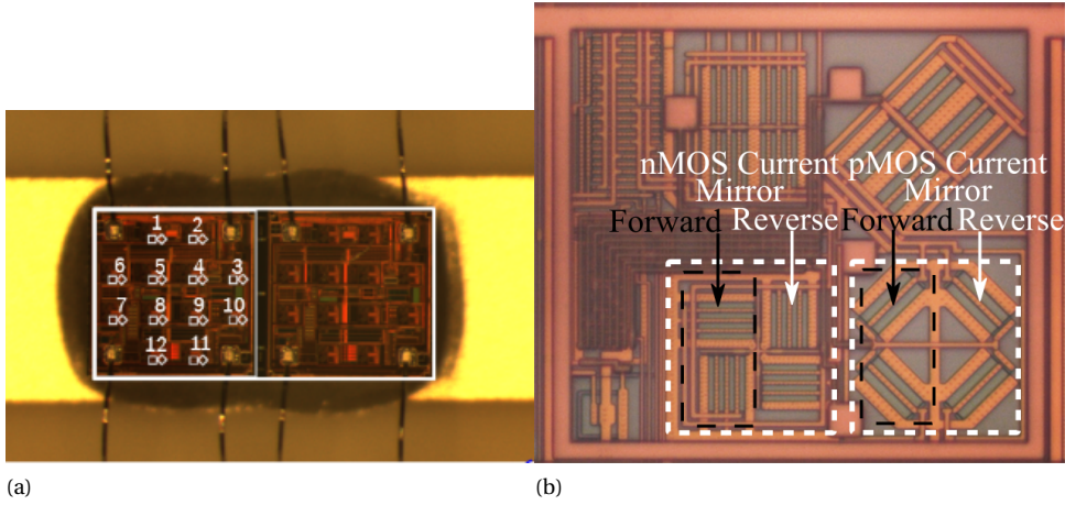
Figure 3.3: Construction of a sensor (a) cells placed in a matrix and (b) single measurement cell containing two current mirrors in a forward and reverse arrangement.
