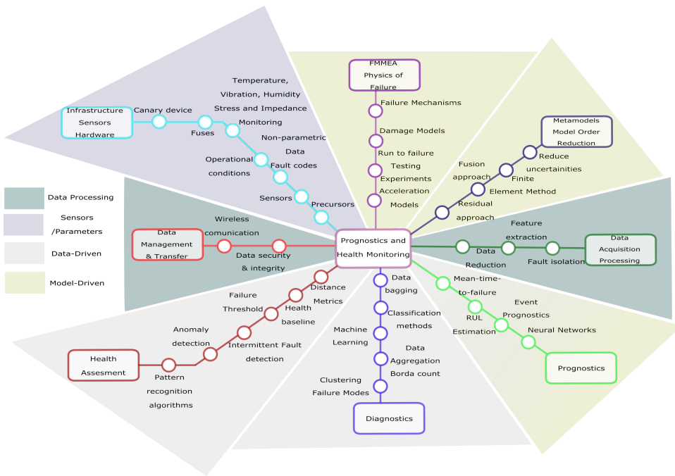
Figure 2.1: PHM for Electronic Systems Metro-Map. The main areas are Data Processing, Sensors, Data-Driven and Model-Driven Approaches.
