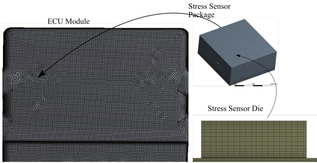
Figure 4.13: Numerical Simulation mesh.
