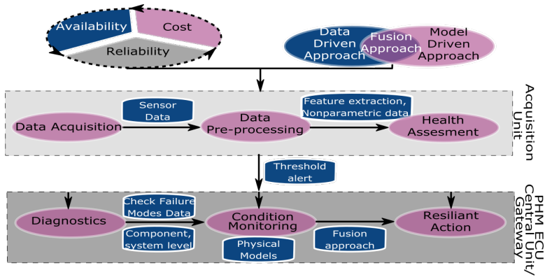
Figure 4.6: Prognostics and Health Monitoring framework.
