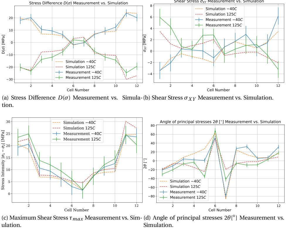
Figure 4.14: FEM examination of the test vehicle. The measurement stress corresponds to relative stress.
