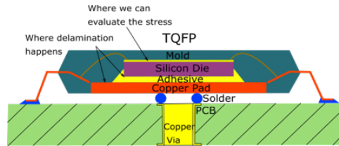
Figure 5.5: Package on PCB cross-section. It shows the main elements of the package and illustrates where the stresses are measured. At the same time, where the delamination usually occurs.
