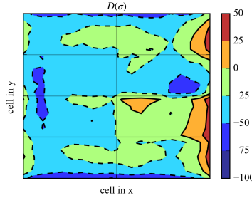
Figure 6.15: MC1_1 TV stress difference at 1400 Cycle.
