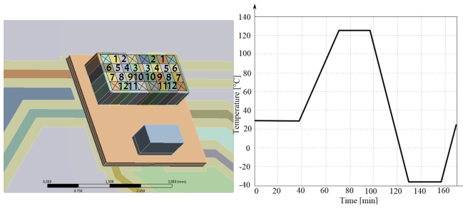
Figure 4.12: Stress sensing cells FEM simulation and the loading conditions.
