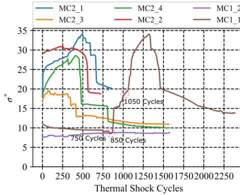
Figure 5.8: Visualization Metric. The sum of absolute stress value change divided by the number of cells in cycle time for MC1 and MC2 . In all samples a stress increase is observed followed by a decrease. Only one sample MC1_2 showed constant sum of absolute stress.
