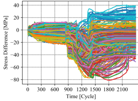
Figure 5.7: MC1_1 TV 480 stress difference sensing cells representation during the experiment. This graph shows the complexity of the stress change during the temperature cycling.
