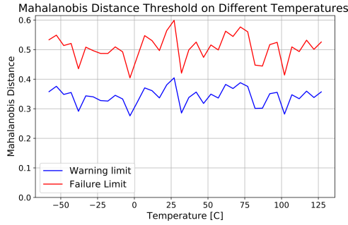
Figure 4.24: Threshold Evaluation performed at all temperatures. Based on this graph a mean can be computed to represent the temperature independent threshold.
