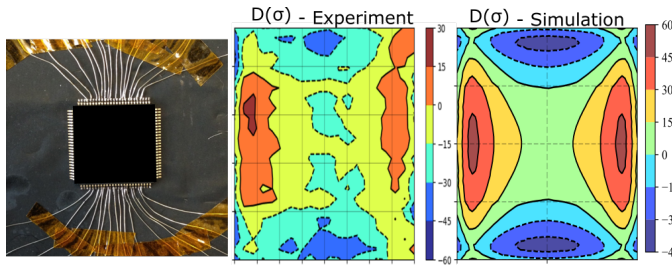
Figure 6.11: TQFP component level mechanical stress at the top of the die measured vs. simulation. Loading condition used in the simulation and measurement is an environmental temperature of -40^\circ and 150^\circ . The stress values at -40^\circ are extracted from 150^\circ stress values.
