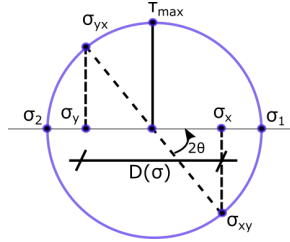
Figure 4.4: 2D Mohr Circle. Describes the relationship between measured and calculated parameters.
