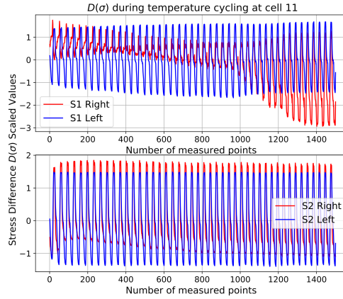
Figure 4.16: Stress evolution of the delamination during temperature cycling of the Sample 1.
