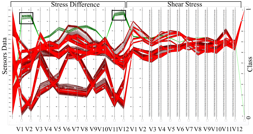
Figure 4.22: The effect of damages on the different sensor readings is shown with parallel coordinates, where the readings of 12 sensor cells are related. It can be seen that the sensor cells V1, V2, V11, V12 with stress difference values capture the effect of the damages (marked with two rectangles).
