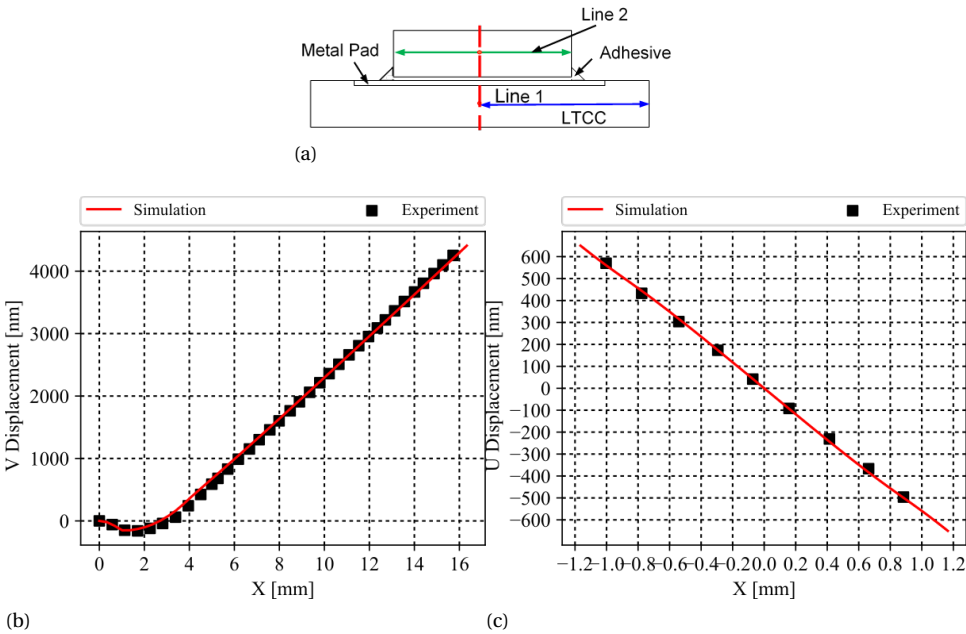
Figure 3.17: Relative local in-plane displacement fringe patterns after apply O/DFM with \beta = 4 at (a) -40^\circ\text{C} (b) at 125^\circ\text{C} .
