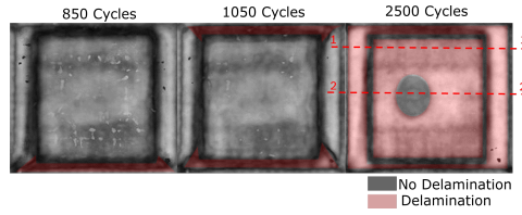
Figure 5.9: SAM of MC1_1 during and after the experiment. Delamination is detected and is depicted in red areas. Two cross-section are performed at the end of the experiment, after 2500 Cycles.
