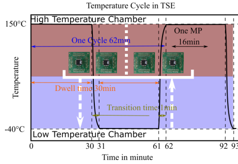
Figure 5.4: Temperature cycle duration. Transition time and the dwell time is briefly specified. The high temperature chamber is shown in red and the low temperature chamber is shown in blue. The transition basket is described in white arrows.
