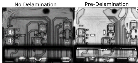
Figure 4.9: Process intended pre-delamination. The left sample follows a standard packaging process, whereas the right sample has delamination created before the injection molding process.
