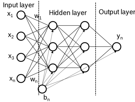
Figure 6.18: Visual representation of an Artificial Neural Network.
