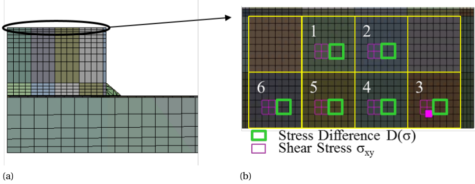
Figure 3.13: Detailed mesh of the sensor chip: (a) side view and (b) top view where the elements used to extract stress are marked.
