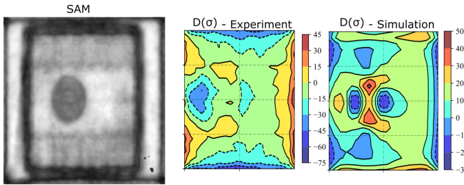
Figure 6.13: Simulation and measured mechanical stress difference at the top of the die of the delaminated MC1_1 TV. Loading condition used in the simulation is an environmental temperature of -40^{\circ} and 150^{\circ} . The stress values at -40^{\circ} are extracted from 150^{\circ} stress values.
