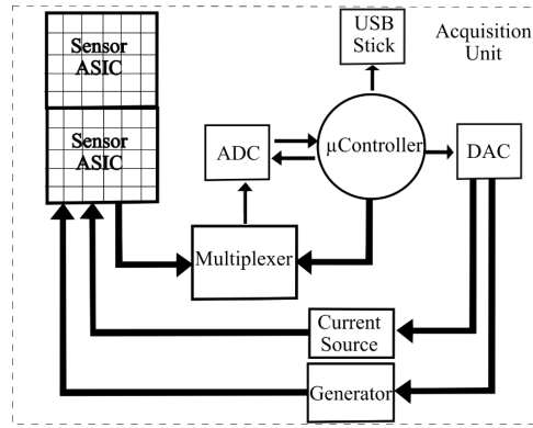
Figure 3.5: Functional scheme of the acquisition unit. The microcontroller first sends the signal to the DAC that regulates the sensor's current and voltage. Then an ADC reads out the sensor response. In addition, a multiplexer is used to switch between different sensors.
