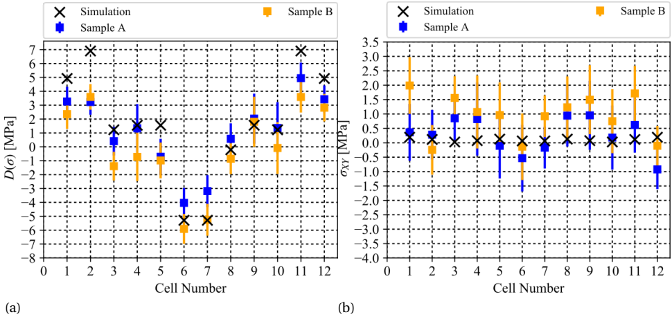
Figure 3.18: Comparison of experimental data and numerical results: (a) the stress difference and (b) the shear stress.
