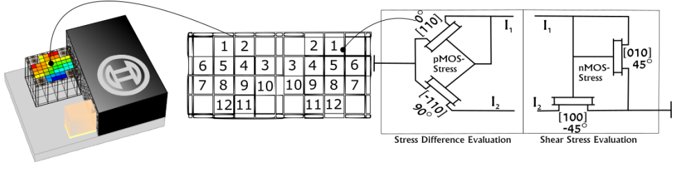
Figure 4.3: Sensor cell numbering in a LGA package. P-mos and n-mos MOSFET channels used to acquire the data.
