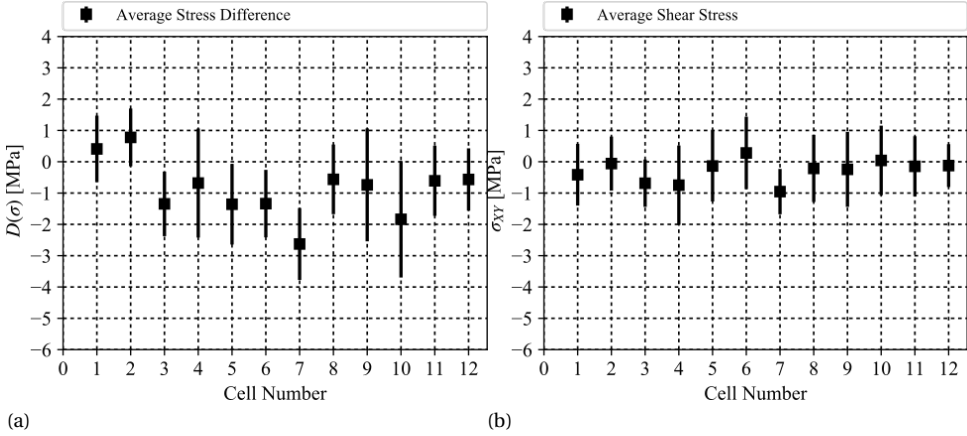
Figure 3.10: Stresses of free standing chips, caused by cooling them from 125^{\circ}\text{C} to -40^{\circ}\text{C} : (a) the stress difference and (b) the shear stress. The error bars show the variations obtained from 12 independent measurements of free-standing chips.
