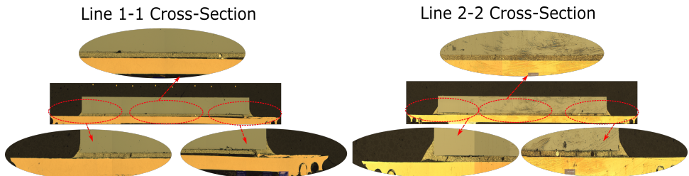
Figure 5.11: Cross-section Failure Analysis of MC1_1 along Line 1-1 and Line 2-2. Crack is present at the interface between molding compound/copperpad and die attach/copper pad along the entire cross-section for Line 1-1, except the middle part in Line 2-2.
