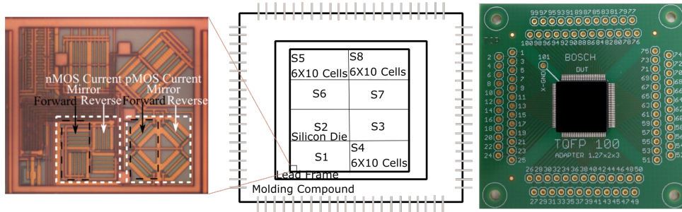
Figure 5.3: Test Vehicle. 8 stress sensors encapsulated in a TQFP package mounted on a PCB. It indicates the sensor location, definition and the number of measuring cells.
