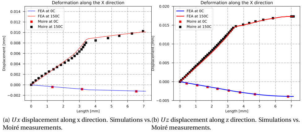
Figure 6.9: FEM ETV model.
