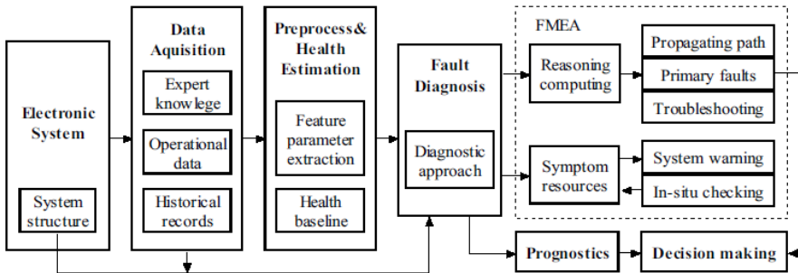
Figure 2.2: Conceptual architecture of PHM-based fault diagnosis for electronics-rich system. [23]
