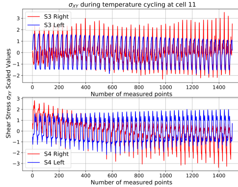
Figure 4.19: Shear Stress evolution of the delamination during temperature cycling of the Sample 2.
