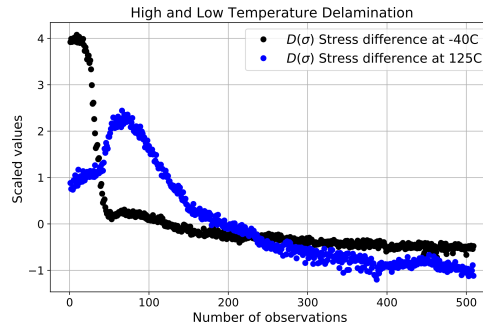
Figure 4.21: Stress Difference evolution during delamination at 125°C and -40°C. More visible changes in stress values are present at low temperature.
