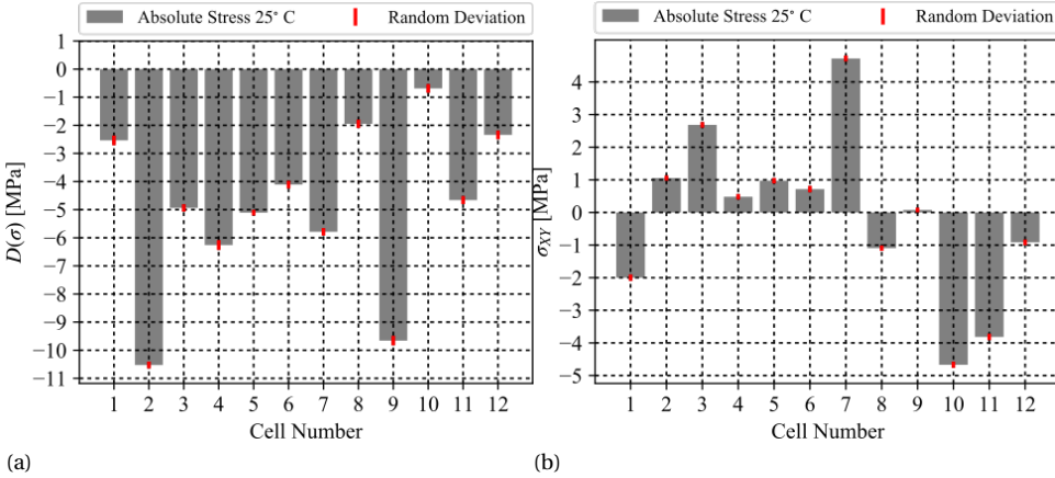
Figure 3.8: (a) Normal stress difference and (b) shear stress obtained from a free standing chip at room temperature. The error bars indicate the random noise determined from 50 measurements.
