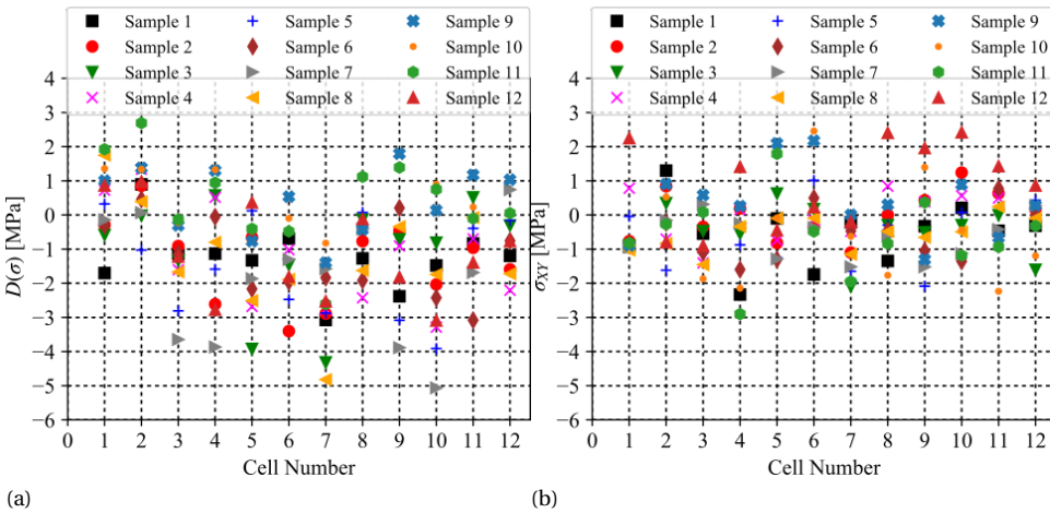
Figure 3.9: (a) Normal stress difference and (b) shear stress obtained from 12 free standing chip at room temperature.
