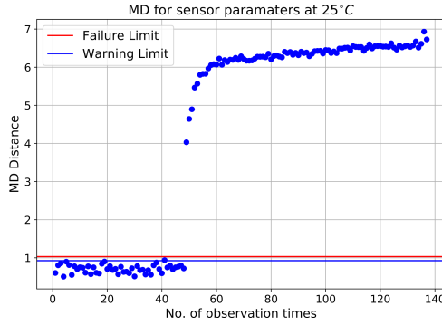
Figure 4.23: Mahalanobis Distance calculated over the 12 cells of the Sample 1 S1. The healthy base is established on the first measurements and every point in measurement is calculated. In this graph there is changes due to the delamination showed in Figure 4.11.
