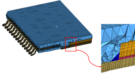
Figure 6.8: Detail on FEM mesh of a quarter model TV TQFP.
