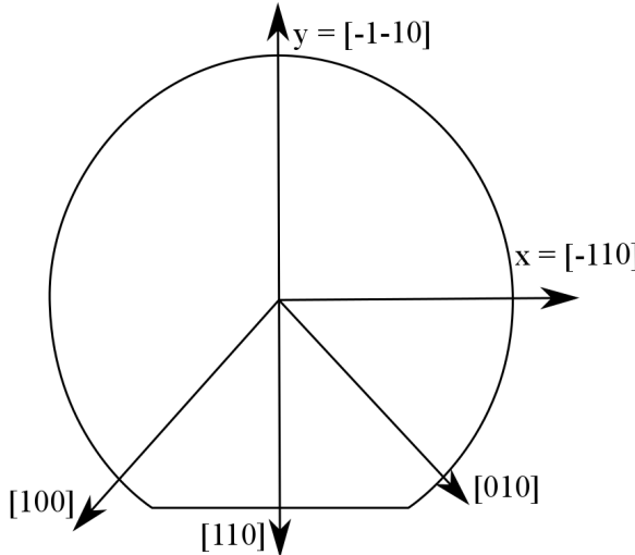
Figure 3.1: Coordinate system for (100) Silicon.
