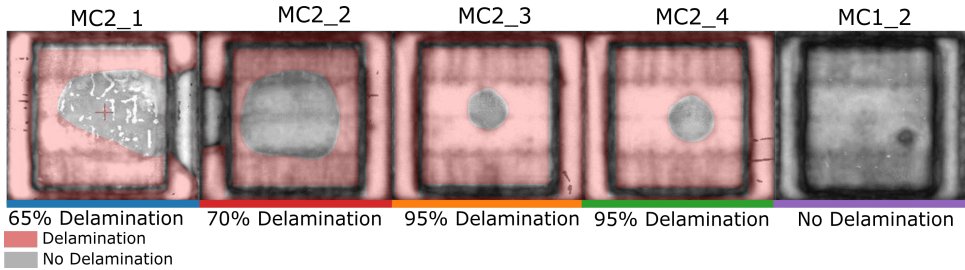
Figure 5.17: SAM Images at the end of the experiments for MC1 and MC2 .
