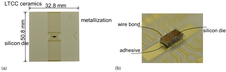
Figure 3.11: LTCC Test Vehicle. The two sensors in a single die is glued on top of an LTCC. The board consists of signal traces that connects the sensor to the exterior pads, on which solder wires are placed.
