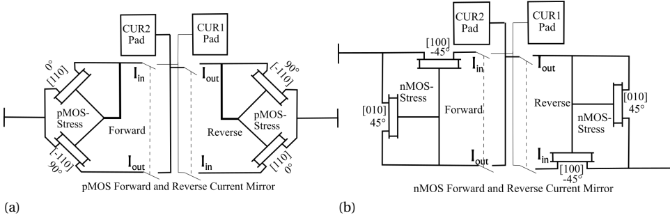
Figure 3.2: Current mirror circuit used for stress measurement (a) pMOS current mirror used for the difference in normal in-plane stress measurement (b) nMOS current mirror used for the xy shear stress measurement.
