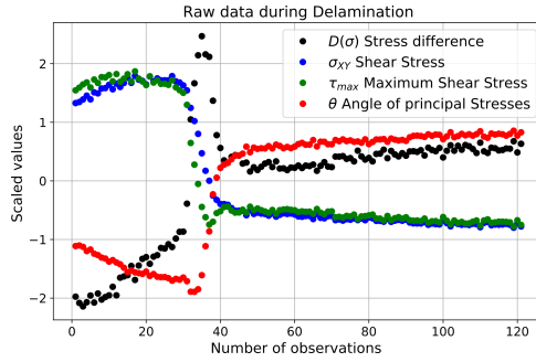
Figure 4.5: Raw data example at room temperature during delamination of the overmolded structure.
