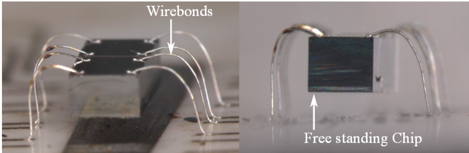
Figure 3.6: Free-standing chip electrical connections. Every each sensor needs four wire connections. The picture depicts two sensors.
