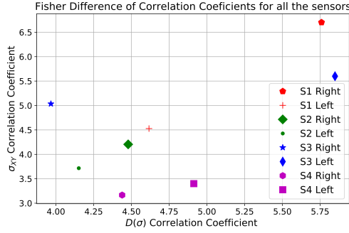
Figure 4.26: Fisher Correlation Coefficient Difference. This difference is performed by using Fisher method of comparing two correlation coefficients. In this case all the sensors correlation coefficient data have been compared with the correlation coefficient as healthy state. The values from the graph represents the z-score values.
