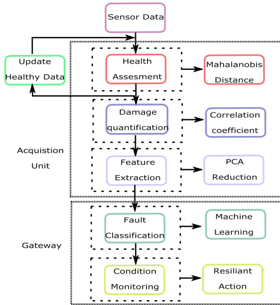
Figure 4.7: Algorithm flowchart.
