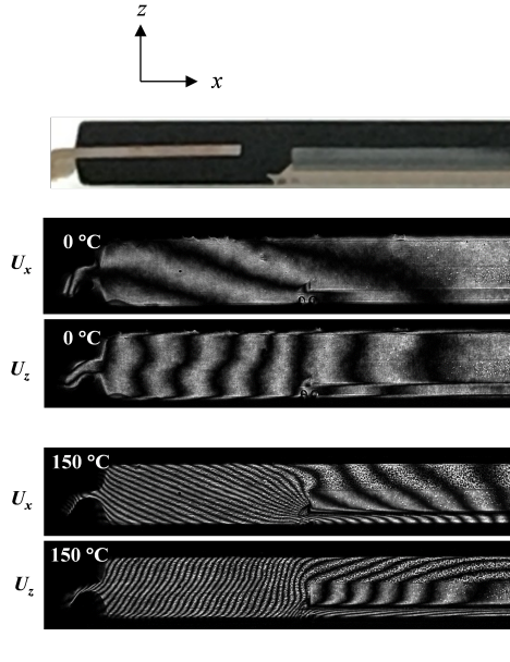
Figure 6.7: U_x and U_z displacement fields of the left-half of the TQFP obtained at 0^\circ and 150^\circ .
