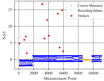
Figure 5.6: Normalized average temperature (NAT) of sensor 3. The temperature is calculated at each cell position and then averaged in one value. The jump in the scaling data is represented by the stop and start of the experiment. A pause explains the orange data in the chamber operation.
