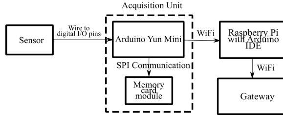
Figure 6.4: Data flow. Arduino Yun Mini collects the data from the sensors, saves the data to a memory card and also sends the data to the Raspberry Pi.
