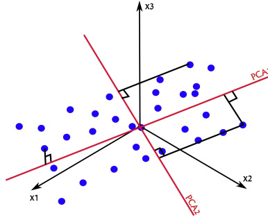
Figure 4.27: A simplified visual representation of the reduced space. Orthogonal projections on the new reduced principal components are depicted.
