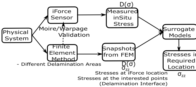
Figure 6.17: Surrogate Modelling.
