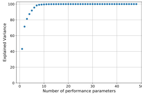
Figure 4.28: Explained variance. It measures the proportion to which PCA model accounts for the data variation.
