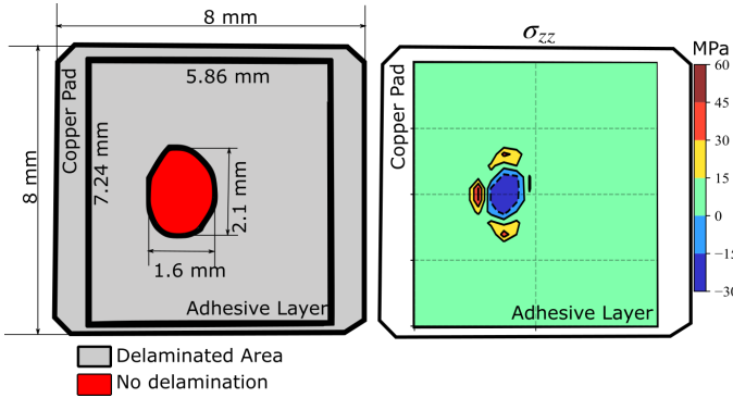
Figure 6.16: Delaminated area versus \sigma_z on simulation dataset. Grey area represents the delaminated area and in the simulation is given as a no contact interface. The red area represents no delaminated area and in the simulation is given as a bonded contact interface.
