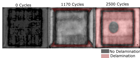
Figure 6.5: MC1_1 TV SAM image before and after the reliability test. The delamination area is shown in red color.
