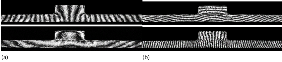
Figure 3.16: Relative local in-plane displacement fringe patterns after apply O/DFM with \beta = 4 at (a) -40^\circ\text{C} (b) at 125^\circ\text{C} .
