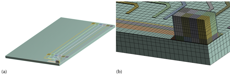
Figure 3.12: Mesh quality used in numerical model. The focus areas are identified by the fine mesh.
