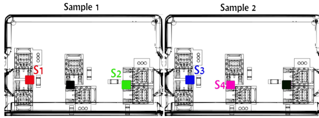
Figure 4.10: The position of each sensor on the Outer molded electronic control unit.
