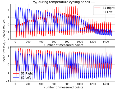
Figure 4.18: Shear Stress evolution of the delamination during temperature cycling of the Sample 1.
