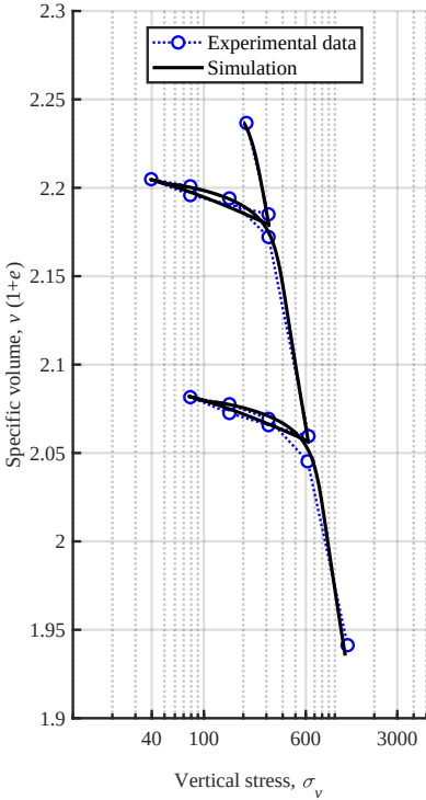
Figure 5.16: Comparison of the model predictions with oedometer experimental data of Suddepong et al. [55]
