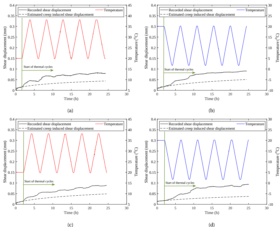
Figure 7.3: Evolution of shear displacement of sand-concrete interface during thermal cycles: : (a) heating cycles at \sigma_n = 50 kPa; (b) cooling cycles at \sigma_n = 50 kPa; (c) heating cycles at \sigma_n = 150 kPa; (d) cooling cycles at \sigma_n = 150 kPa
