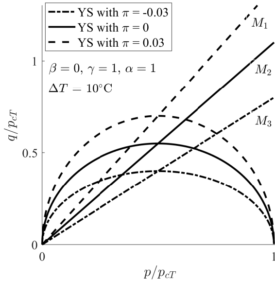
Figure 2.9: Effect of parameter \pi on the shape and size of the yield surface
