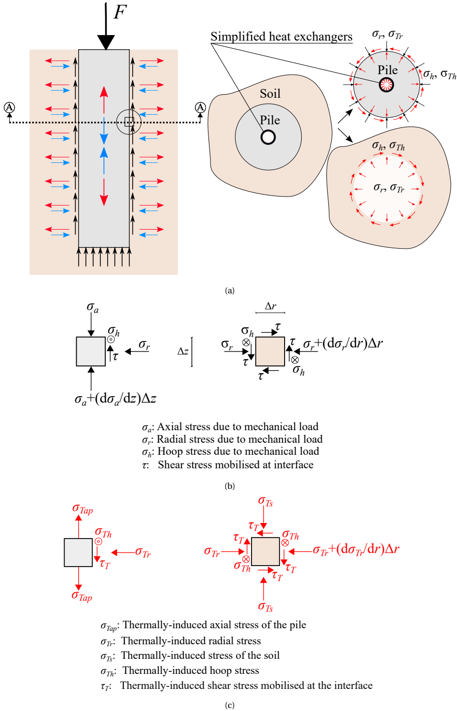
Figure 1.1: (a) Stresses developed during the deployment of the energy pile; (b) mechanical stresses; (c) thermally-induced stresses
