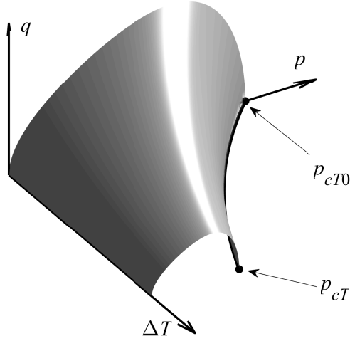
Figure 4.2: Yield surface in p - q - \Delta T space with M_c = 1.00 , \mu_0 = 0.001 , \pi^* = 0 and \alpha = \gamma = 0.5
