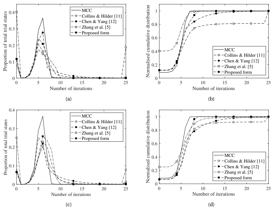
Figure 3.12: Distribution of number of iterations for linear elasticity in terms of the proportion of the total trial states for a given number of iterations and normalised cumulative distribution for: (a) and (b), tear-shape type I yield surface; (c) and (d), tear-shape type II yield surface.
