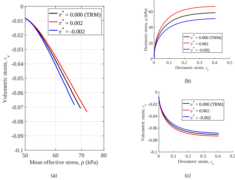
Figure 4.13: Effect of parameter \pi^* on the material's thermomechanical response in triaxial test (a) \epsilon_v vs. p ; (b) q vs. \epsilon_s ; (c) \epsilon_v vs. \epsilon_s
