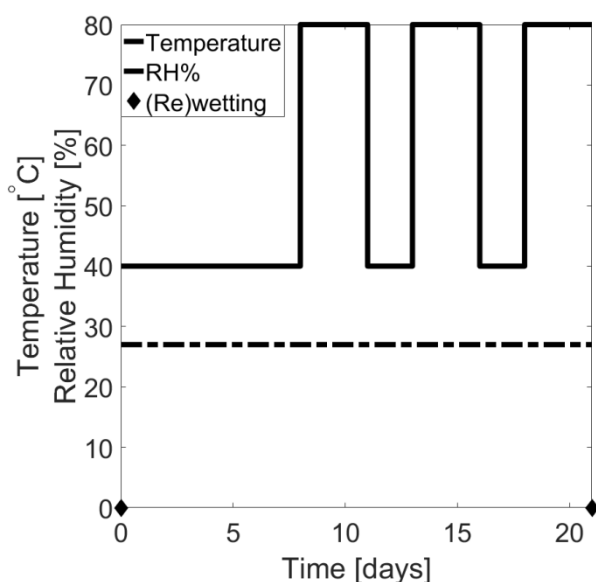
Figure 1: Temperature and RH cycles used in the accelerated salt weathering test. This entire cycle was repeated 5 times.
