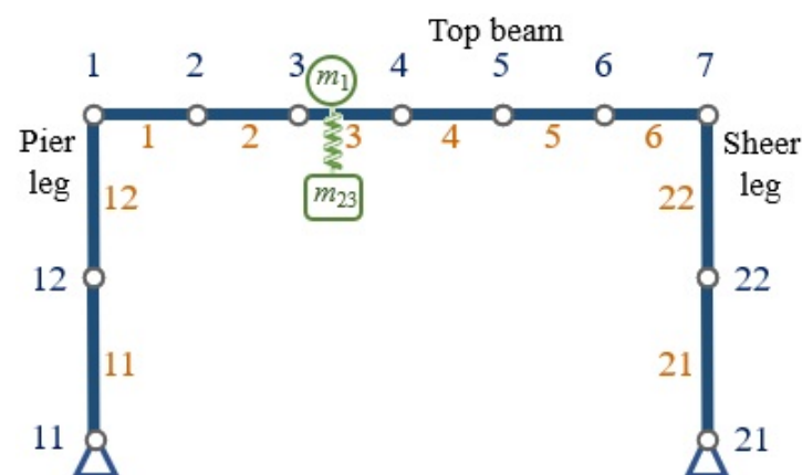
Figure 2. The meshing of the gantry crane (FE model) with the mass moving on the structure.
