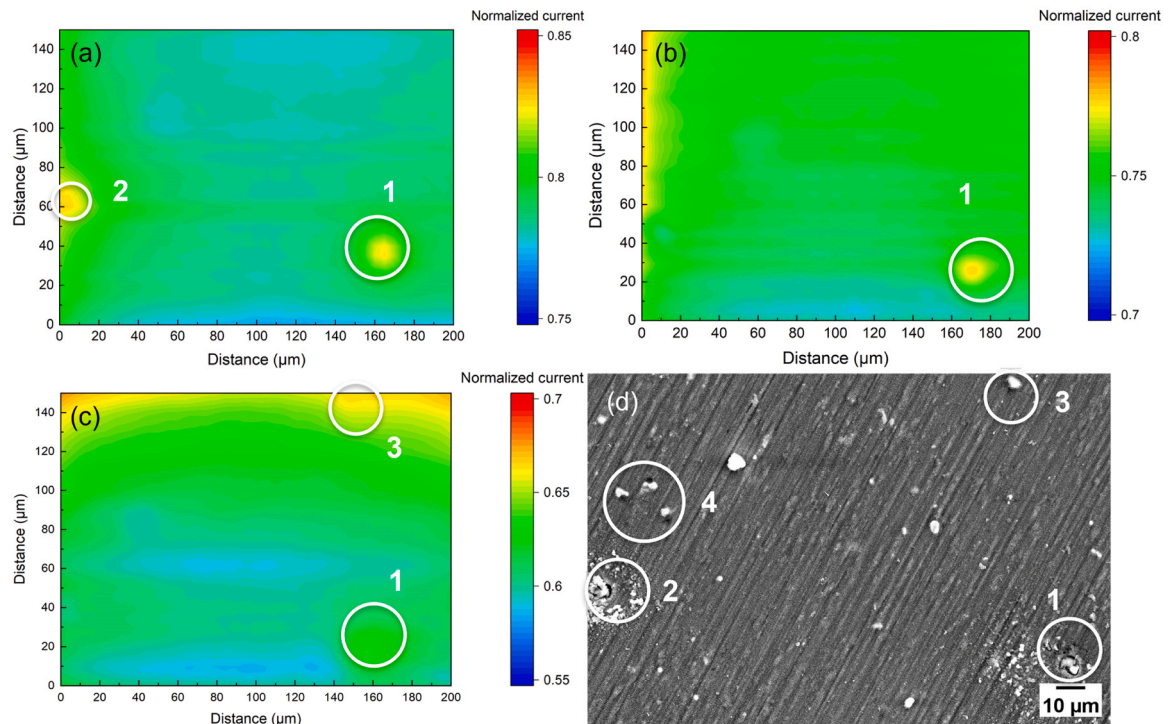
Fig. 7. SECM mapping of a fixed scanning area over a 36 h ambiently-aged lithium-based conversion layer during re-immersion in a 0.01 M NaCl electrolyte containing 2 mM FcMeOH. The scanning time duration is (a) 0.5–1.5 h, (b) 4.5–5.5 h, (c) 8.5–9.5 h. (d) Corresponding SEM micrograph.
