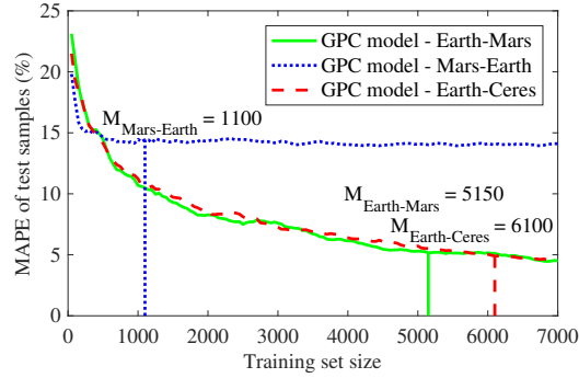
Figure 2: Relationship between MAPE of test samples and number of training samples for GPC models for all three test cases
