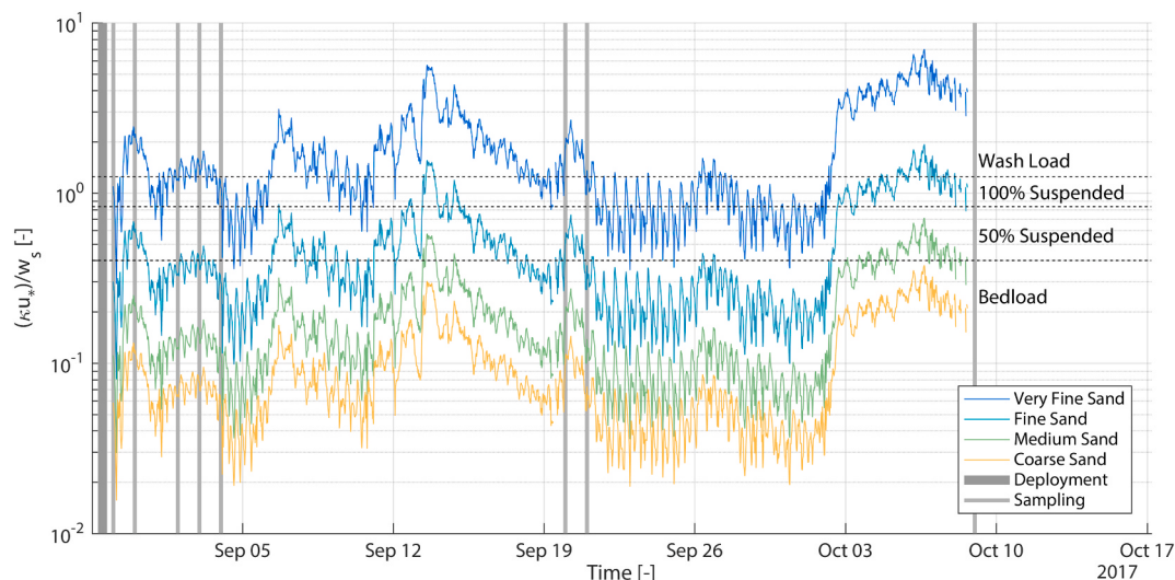
Fig. 10. Inverse Rouse number ( ku^*/w_s ) and transport mode for each sediment class. Calculated using the method of Soulsby (1997) from wave and near-bed velocity measurements taken by a downward-facing ADCP-HR near the tracer source (mounted 0.5 m above the seabed). Tracer sampling dates are indicated by grey bars.
