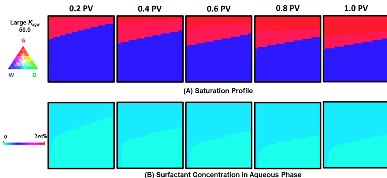
Fig. 5. Case III: Continuous \text{CO}_2 (with dissolved surfactant) injection to displace water with large partition coefficient of K_{sgw} = 50.0 (A) Saturation profile indicating that the foam strength is insufficient to keep \text{CO}_2 from overriding the reservoir; (B) Surfactant concentration profile indicating that the surfactant concentration in the aqueous phase is highly diluted.
