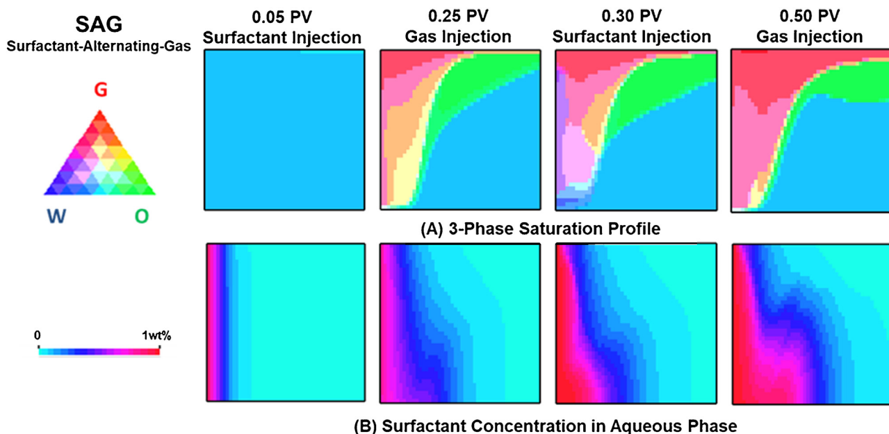
Fig. 8. Case B: Surfactant-alternating-gas. (A) 3-phase saturation profile indicating that the gas mobility is reduced by foam in presence of surfactant and the sweep efficiency is greatly improved from WAG injection. (B) Surfactant concentration profile indicating that significant surfactant drains by gravity before the CO 2 slug catches up. (For interpretation of the references to colour in the text, the reader is referred to the web version of this article.)
