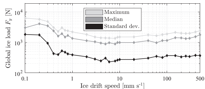
Fig. 4. Ice loads from rigid indenter tests for cold model ice. Rigid experiments were performed with an aluminum pile ( D = 200 mm) and an ice thickness of 25 mm.
