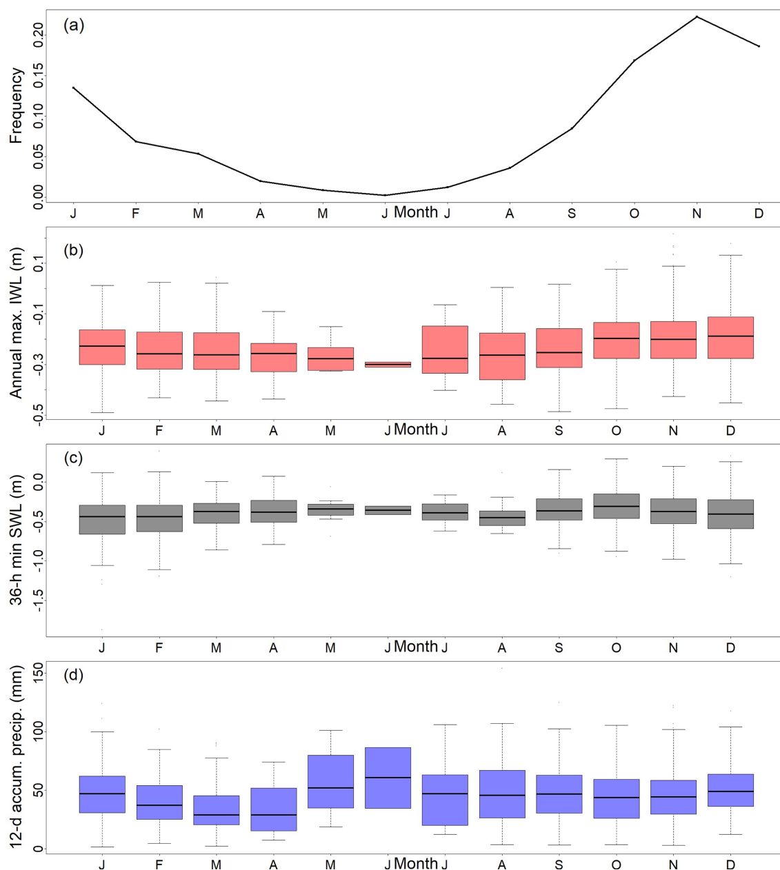
Figure 6. Frequency of WL_{\max} events occurring each month (a), monthly mean of WL_{\max} (b), S^T_{36h,min} (c), and P_{12d,acum} (d).
