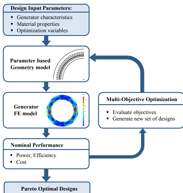
Figure 3: Generator design optimization procedure.
