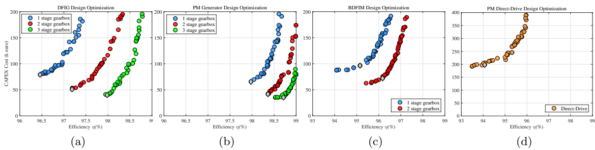
Figure 4: Generator design optimization results for a 3.2 MW wind turbine drive-train
