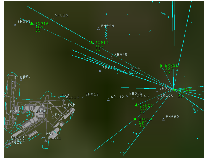
Figure 3. Amsterdam Environment With Geofences in BlueSky [12] ATC simulator
