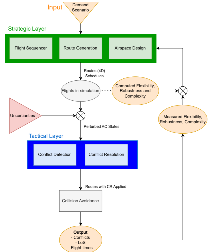
Figure 2. Separation Management System Feedback Model
