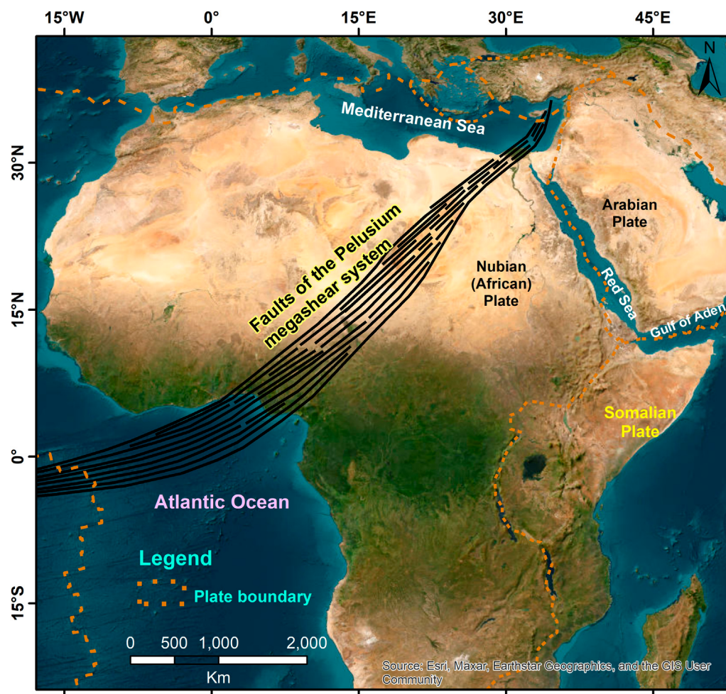
FIGURE 15 Distribution pattern of the faults of the PMS across Africa (Modified after Neev et al., 1982 ).
