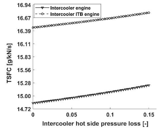
Figure 10: Effect of intercooler hot side pressure loss on: a) Specific Thrust in kN.s/kg; b) TSFC (Thrust Specific Fuel Consumption) in g/kN/s.
