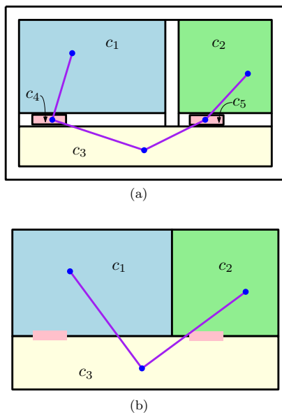
Figure 2. Two ways to model cells in an IndoorGML model. (a) 5 cells are present since doors (pink cells) are explicitly modelled. (b) The doors are not cells, their presence can be inferred by the fact that the navigation graph has an edge between 2 cells.
