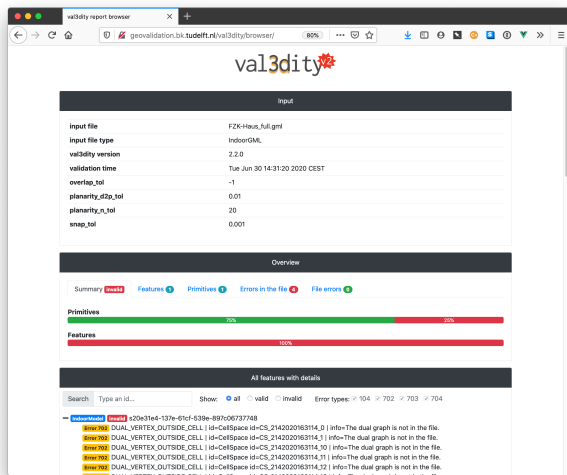
Figure 5. The web-based validation report browser.
