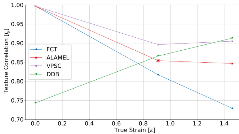
Fig. 8. Texture direct correlation [ J_d ] for scenario-II. Texture correlation quantification between deformation textures obtained with every CP models with respect to experimentally measured deformation textures. [ J_d ] as a function of the equivalent strain.
