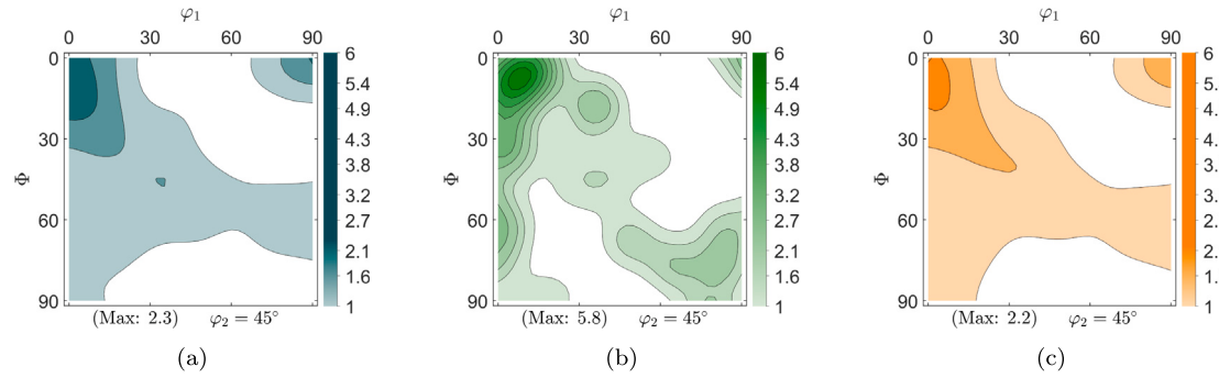
Fig. 13. Input textures for the CP simulations. (a) input ODF for MFCP scenario-II. (b) input ODF for DDB simulation scenario-I and II. (c) Experimentally measured ODF of the as-received material.
