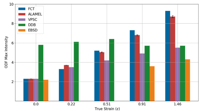
Fig. 10. ODF maximum intensities resulting from scenario-II.
