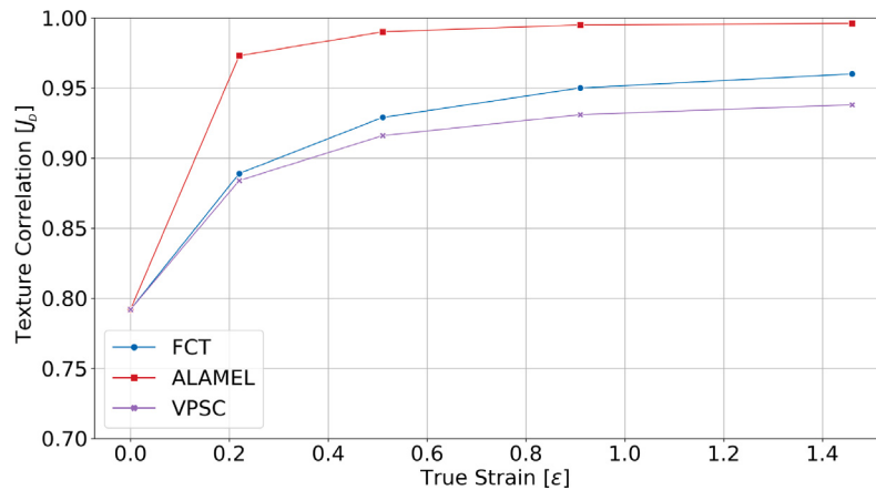
Fig. 11. Texture direct correlation [J_d] for deformation textures for the MFCP models. Comparison between deformation results obtained in scenario-I and scenario-II. [J_d] as a function of the equivalent strain.
