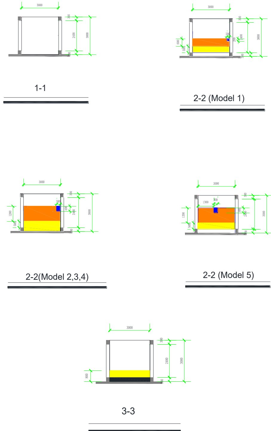
Figure 5.9 Cross-sections (Side Breach; Middle Breach)
