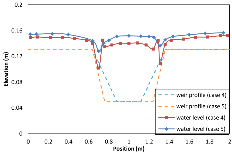
Figure 3.13 Water level in compound weir flow condition ( Q = 50 \text{ l/s} )
