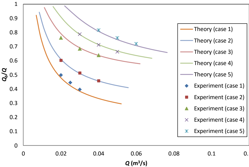
Figure 3.16 Comparison of theory predictions and laboratory measurements on discharge distribution
