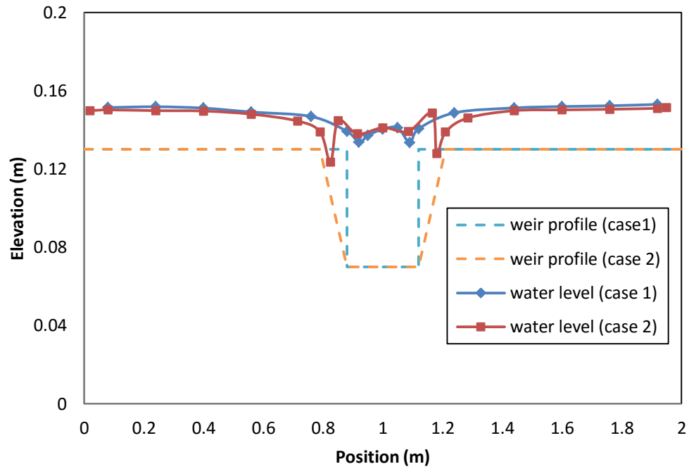
Figure 3.12 Water levels in compound weir flow condition ( Q = 30 \text{ l/s} )
