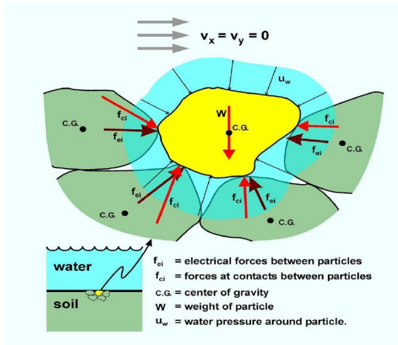
Figure 4.3 Forces upon the soil particle in hydrostatic condition (after Briaud et al. , 2008)
