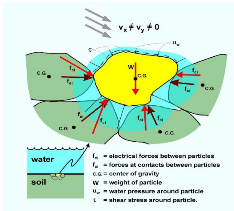
Figure 4.4 Forces upon the soil particle in flow condition (after Briaud et al. , 2008)
