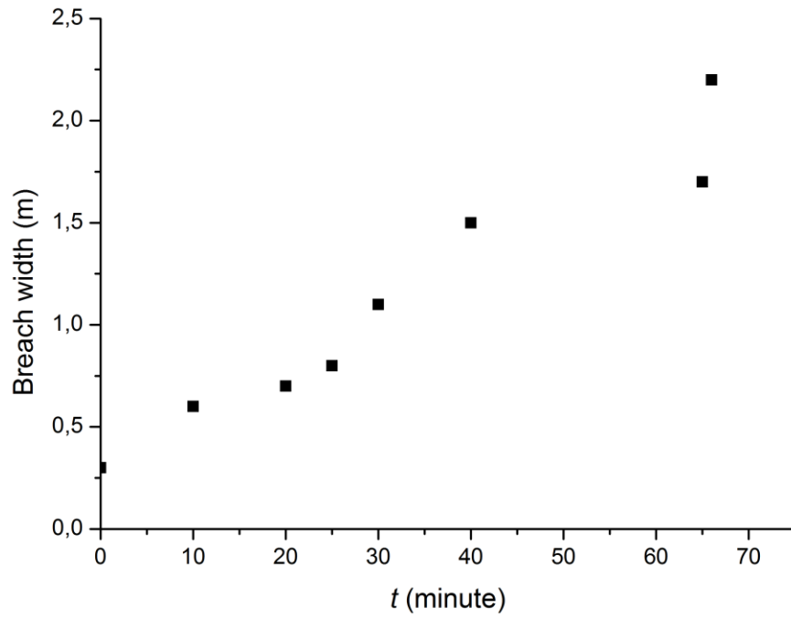
Figure 5.42 Breach lateral migrations in Run 4
