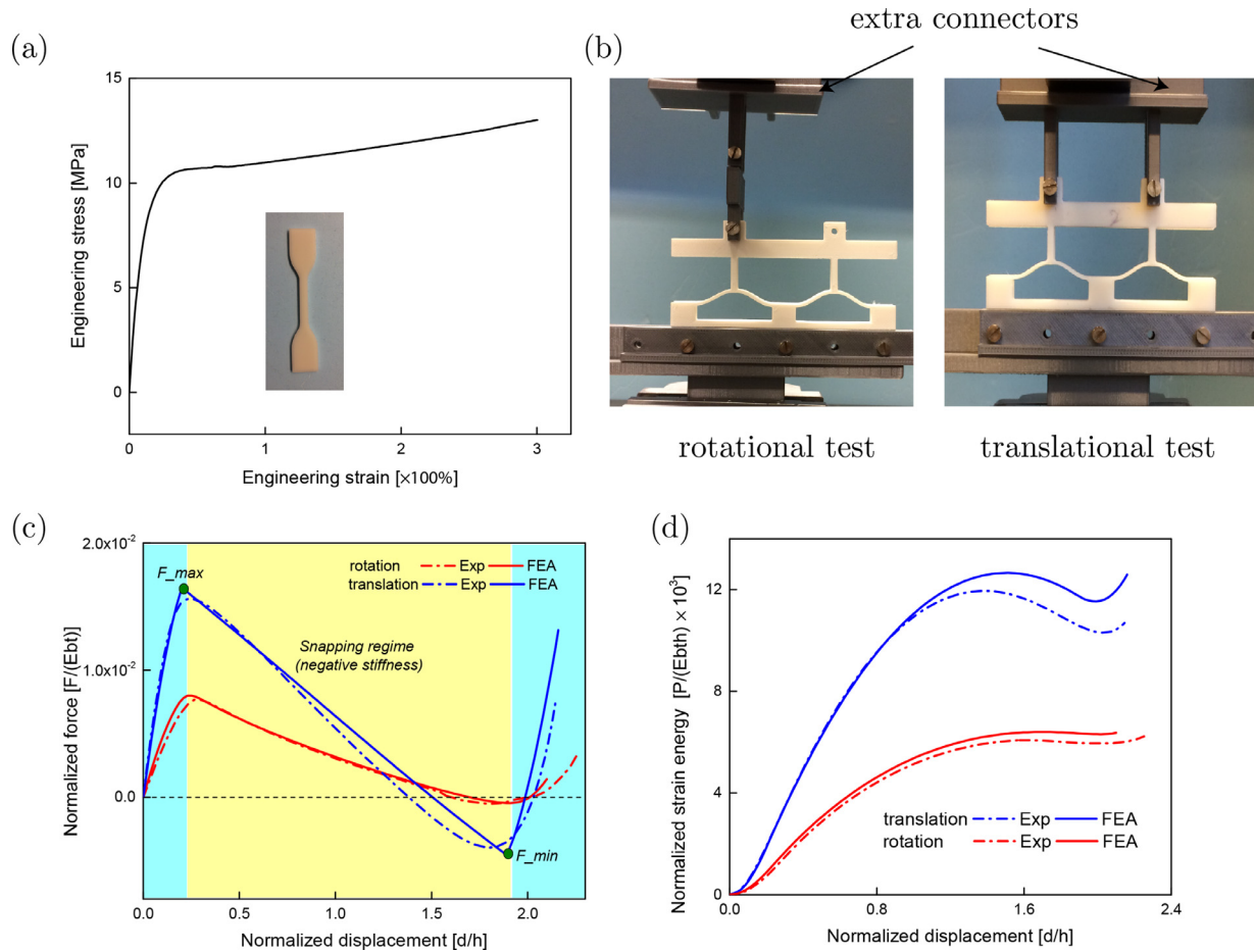
Fig. 2. Characterization of snap-through transitions of the unit cell. (a) Stress-strain results for the material we used. (b) Experimental setup for measuring rotational (left) and translational (right) transitions. Samples are clamped at the bottom and connected to the printed part at the top. (c) Normalized load-displacement curves of snap-through transitions. The blue regions represent positive stiffness phases while the yellow area stands for the snapping phase, exhibiting negative stiffness. F_{max} and F_{min} represent the maximal and minimal force of each load-deflection curves, respectively. (d) Evolution of the normalized strain energy of the unit cell during the uniaxial loading.
