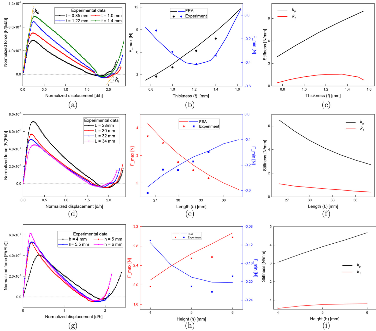
Fig. 3. The influence of t , h , and L on rotational responses. (a)–(c): The effect of t on rotational transitions. (a) shows experimentally measured load-displacement curves for specimens with different thickness. k_0 and k_1 are defined as the slope of tangent line (orange color) at two stable locations (the initial and rotational state). (b) presents F_{max} and F_{min} of force-displacement curves as a function of thickness. The positive sign of F_{min} indicates that the rotational stable state does not exist. (c) represents the change of k_0 and k_1 when varying thickness in FEA. (d)–(f): The effect of L on rotational transitions. (g)–(i): The effect of h on rotational transitions.
