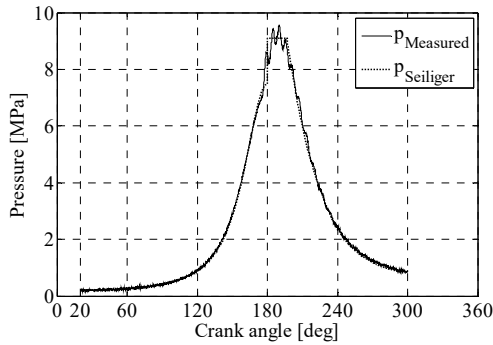
(a) In-cylinder pressure (point A)
