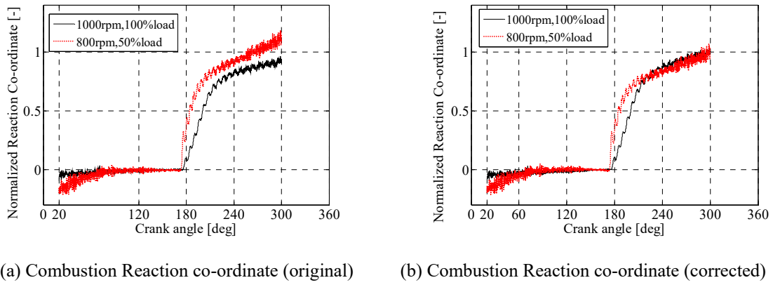
Fig. 5 Combustion Reaction co-ordinate
