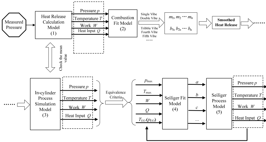
Fig. 3 Flow chart of the overall simulation procedure to calculate Seiliger parameters, ref to (Ding Y, 2011)
