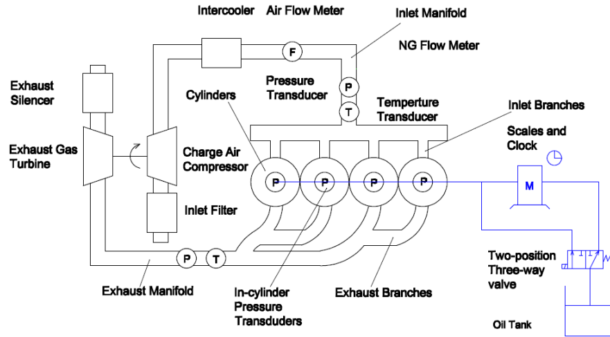
Fig.2 Schematic diagram of in-cylinder pressure measurement test bed
