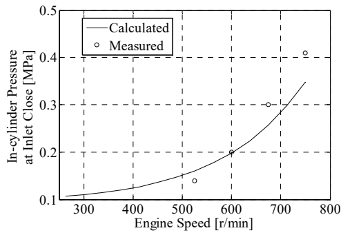
(e) In-cylinder Pressure at IC
