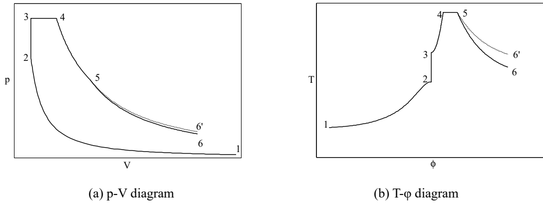
Fig.1 six-point Seiliger process definition [Ding Y, 2011]
