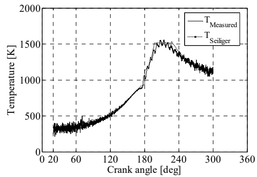
(b) Cylinder temperature (point A)
