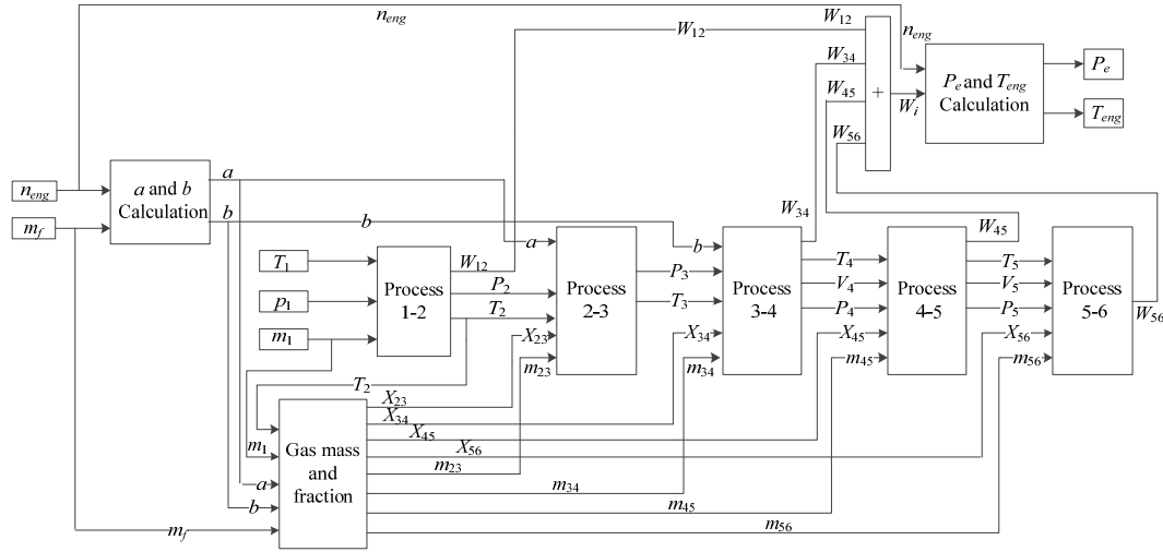
Fig.11 Mean value model of the in-cylinder process in SIMULINK
