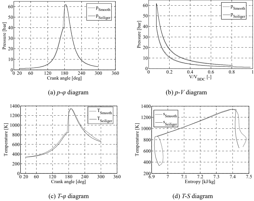
Fig. 7 Comparison of fitted Seiliger cycle with smoothed measurement
