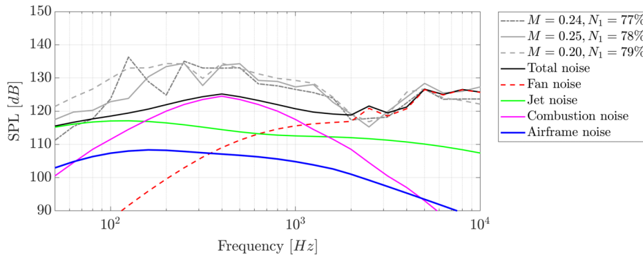
Fig. 17 Comparison of the predicted (in color) and measured (in gray) spectra of the A320 for takeoff.
