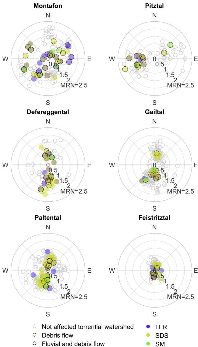
Fig. 10. Overview of the torrential watersheds of the study regions according their mean aspect and Melton Ruggedness Number (MRN). Colored points mark the sub-watersheds (i.e. torrential watersheds) of a study region which produced torrential events. Gray colored points mark sub-watersheds where no event was registered during the study period.
