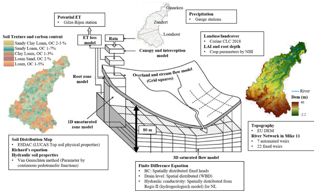
Figure 3.2. Schematic representation of MIKE SHE hydrological model for Aa of Weerijds
