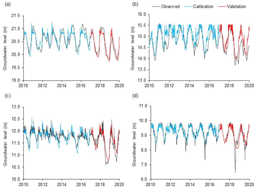
Figure 3.5. Observed and simulated Groundwater levels during the calibration and validation period at locations (a) GW13 (1-0334), (b) GW11 (1-0170), (c) GW9 (5219), (d) GW7 (B50C0079)
