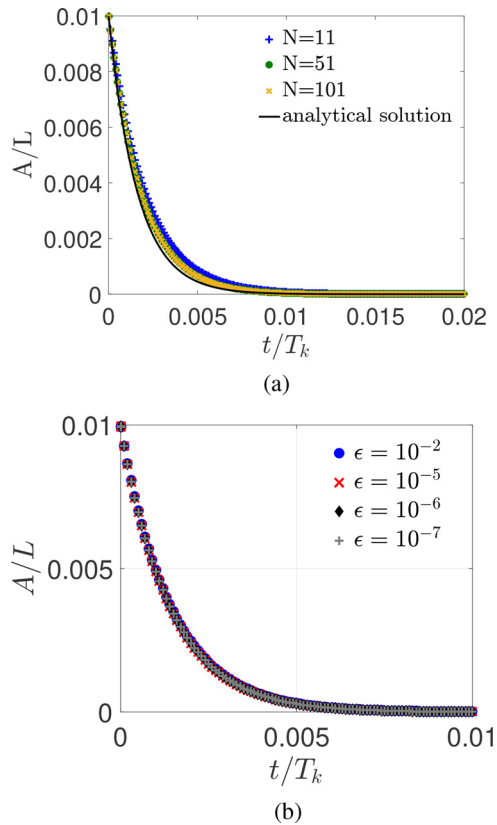
FIG. 3. (a) Relaxation of the displacement amplitude A(t) for different discretization point numbers N . The numerical results approach the analytical solution as N increases. (b) Relaxation of the displacement amplitude A(t) for different values of the regularization parameter \epsilon .
