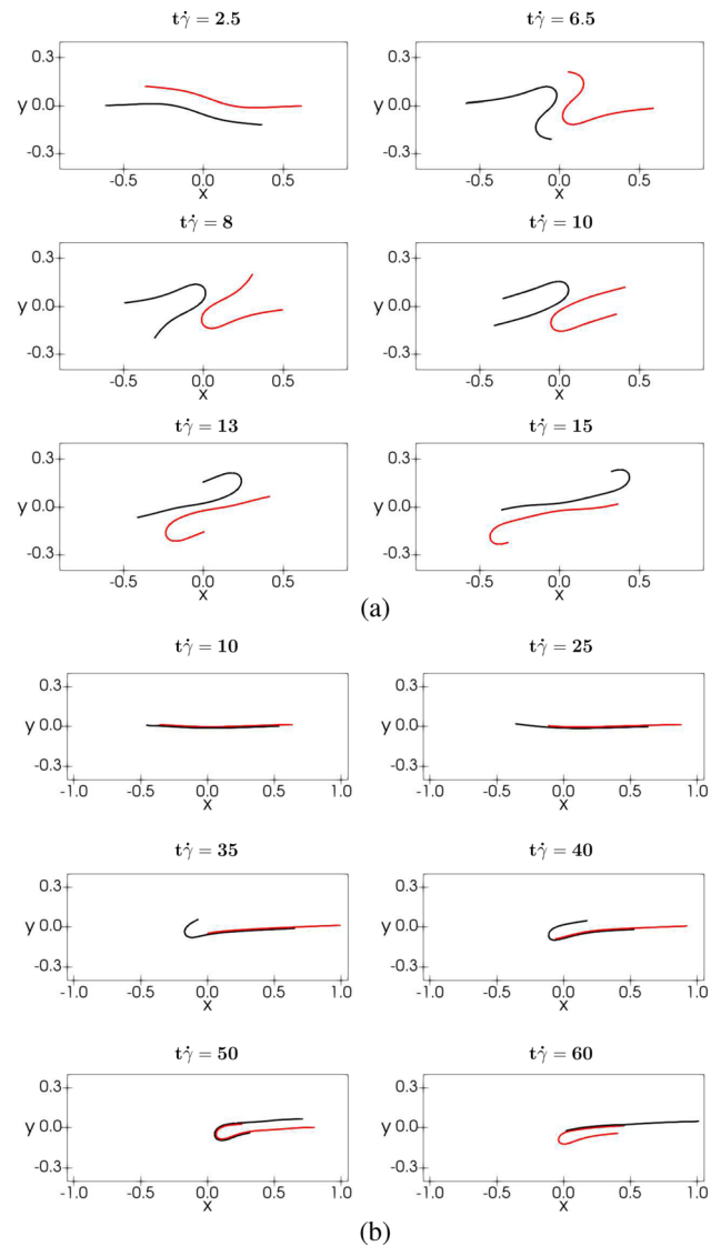
FIG. 9. (a) Interaction between two sheets for an initial odd perturbation ( a_0/L = 0.05 ), initial distance d_0/L = 0.1 and \dot{\gamma}_L = 1000 . (b) Initial even perturbation ( a_0/L = 0.05 ), initial distance d_0/L = 0.01 and \dot{\gamma}_L = 2000 . For a video of the simulations, see supplementary material.
