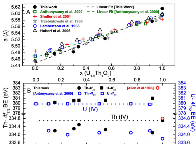
Fig. 5. Lattice parameter of U_{1-x}Th_xO_2 films versus x obtained in this work and compared to literature data obtained on bulk compounds (A). Th-4f 7/2 and U-4f 7/2 Binding energy in U_{1-x}Th_xO_2 films obtained in this work and compared to literature obtained on bulk compounds (B).
