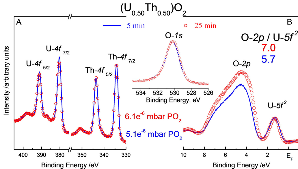
Fig. 3. The influence of the deposition time on the U-4f and Th-4f core level spectra (A) and on the HeI valence band spectra (B) for U_{0.50}Th_{0.50}O_2 .
