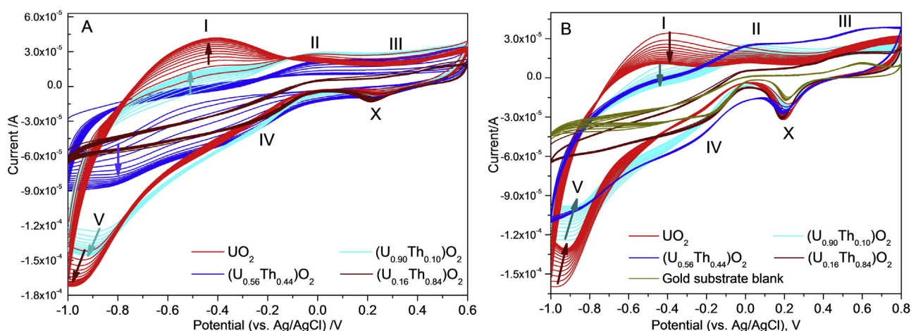
Fig. 7. Cyclic voltammetry for U_{1-x}Th_xO_2 ( x = 0, 0.10, 0.44, 0.84, 1 ) films from the 3rd up to the 15th cycle in the range of -1 V to 0.6 V (A). Cyclic voltammetry for U_{1-x}Th_xO_2 ( x = 0, 0.10, 0.44, 0.84, 1 ) films for higher potential window up to 0.8 V (vs. Ag/AgCl) and gold substrate cycles (yellow lines) (B). (For interpretation of the references to colour in this figure legend, the reader is referred to the web version of this article.)
