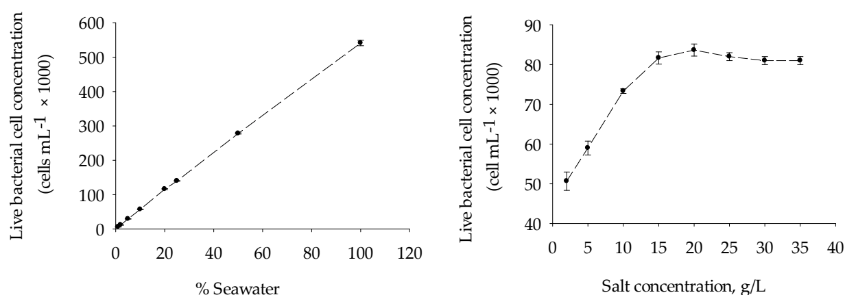
Figure 3. (a) Reproducibility and precision of flow cytometry for measuring live bacterial cell concentration in seawater sample and (b) bacterial live cell enumeration by FCM after inoculation of the same concentration seawater bacteria (collected from North seawater) to the ASW prepared at different concentrations (0–35 g/L) by varying the concentration of Na + and Cl - (Table 2).
