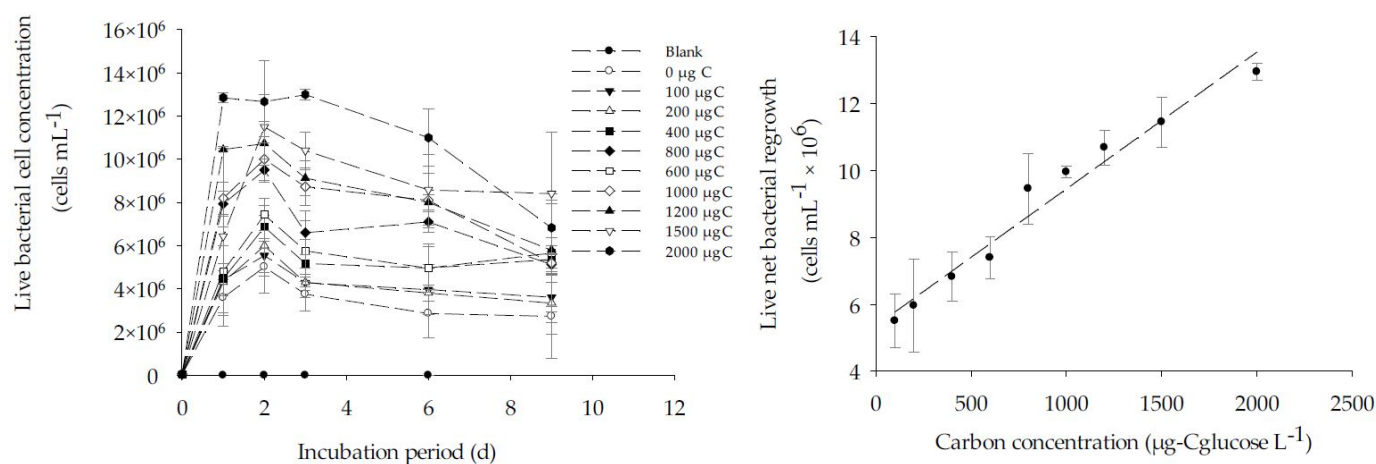
Figure 6. The correlation between the live bacterial net regrowth and carbon concentration (0–2000 µg-C glucose /L) in real seawater sample.
