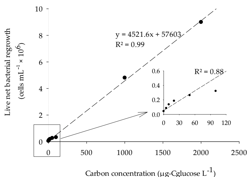
Figure 5. The correlation between the live bacterial net regrowth and carbon concentration (0–2000 \mu\text{g-C}_{\text{glucose}}/\text{L} ) in ASW sample.
